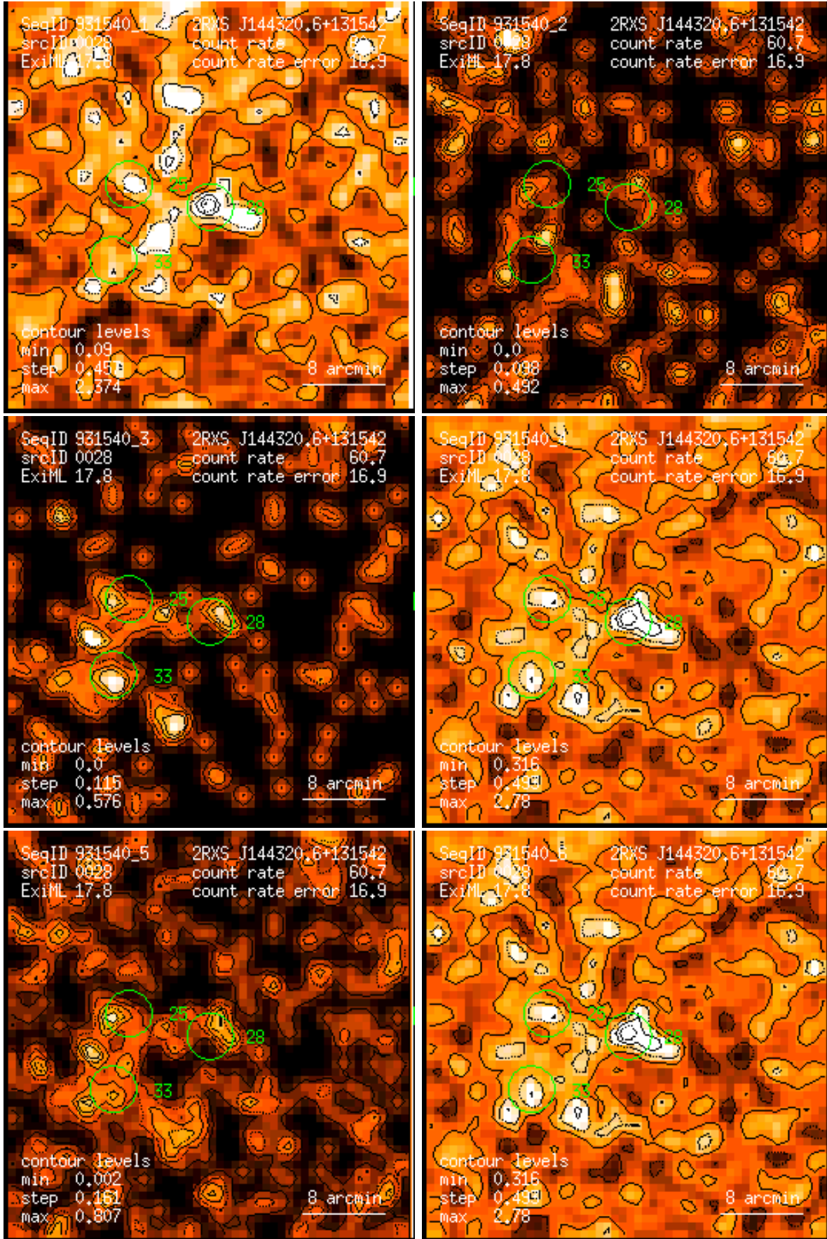
Figure 28: RASS 931540: detection 0028: band rate images, Gaussian filter: (1) PSPC channels 11 – 41, (2) 52 – 90, (3) 91 – 201, (4) 11 – 235, (5) 52 – 201, (6) 11 – 201. Broad band rates in counts/ks. Band rate contour levels in counts/ks/arcmin 2 .
