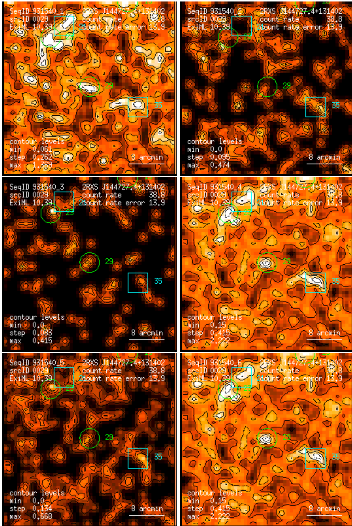
Figure 29: RASS 931540: detection 0029: band rate images, Gaussian filter: (1) PSPC channels 11 – 41, (2) 52 – 90, (3) 91 – 201, (4) 11 – 235, (5) 52 – 201, (6) 11 – 201. Broad band rates in counts/ks. Band rate contour levels in counts/ks/arcmin 2 .
