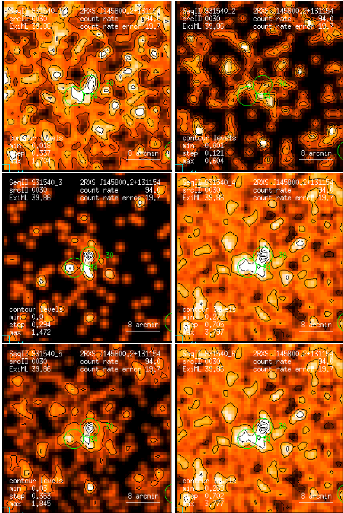
Figure 30: RASS 931540: detection 0030: band rate images, Gaussian filter: (1) PSPC channels 11 – 41, (2) 52 – 90, (3) 91 – 201, (4) 11 – 235, (5) 52 – 201, (6) 11 – 201. Broad band rates in counts/ks. Band rate contour levels in counts/ks/arcmin 2 .
