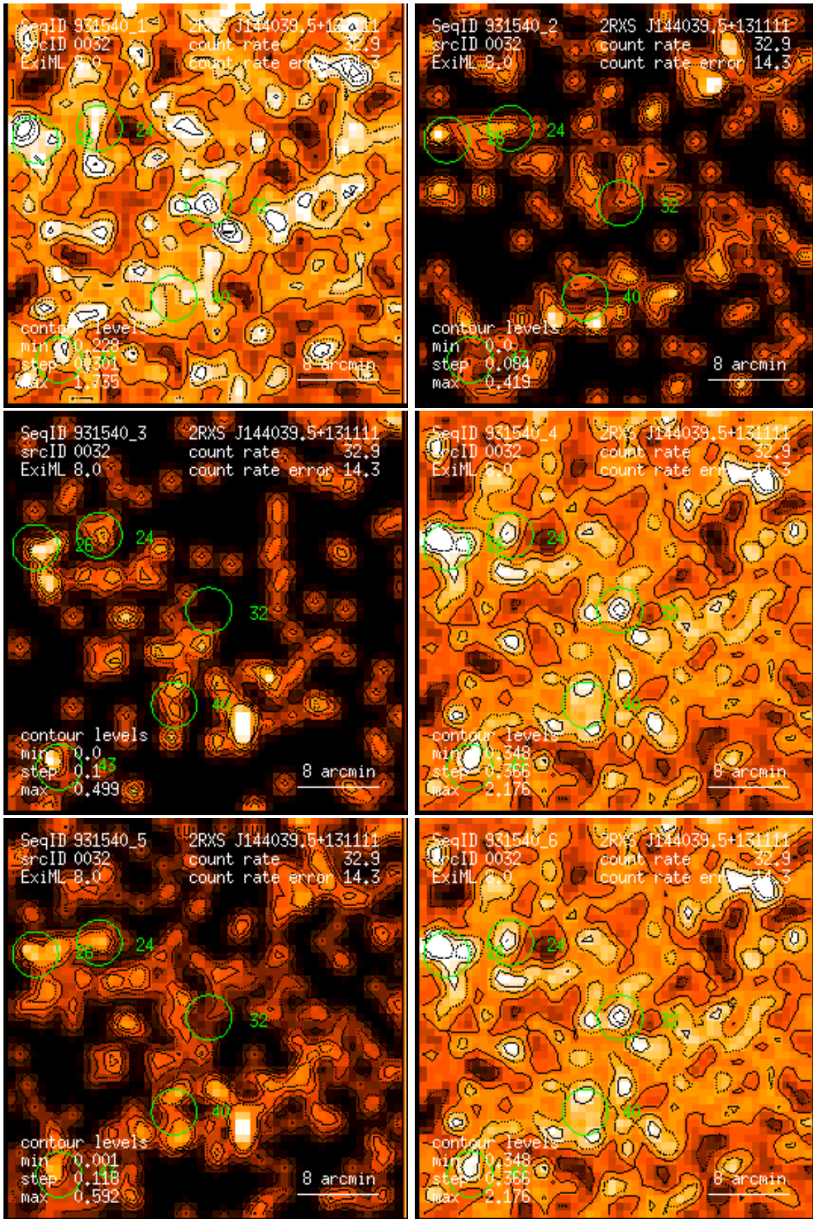
Figure 32: RASS 931540: detection 0032: band rate images, Gaussian filter: (1) PSPC channels 11 – 41, (2) 52 – 90, (3) 91 – 201, (4) 11 – 235, (5) 52 – 201, (6) 11 – 201. Broad band rates in counts/ks. Band rate contour levels in counts/ks/arcmin 2 .
