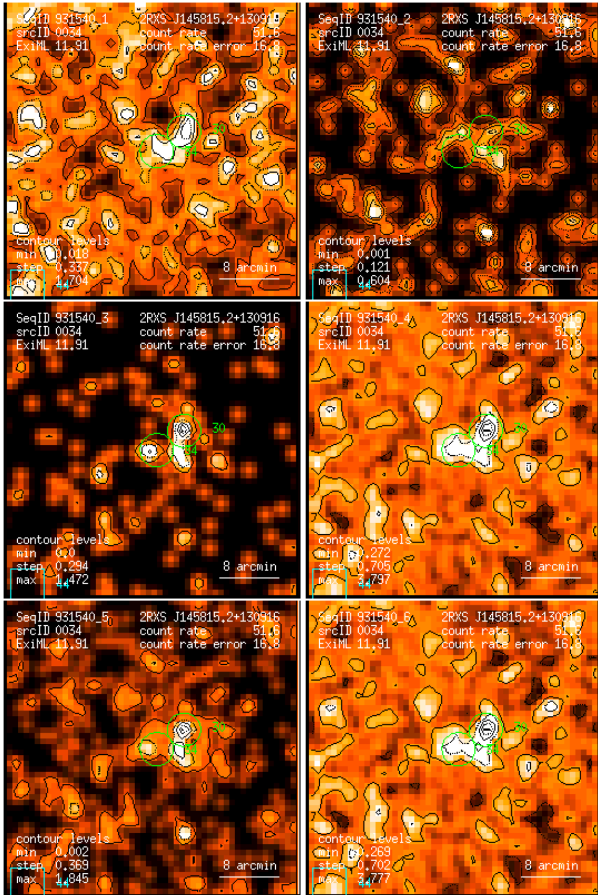
Figure 34: RASS 931540: detection 0034: band rate images, Gaussian filter: (1) PSPC channels 11 – 41, (2) 52 – 90, (3) 91 – 201, (4) 11 – 235, (5) 52 – 201, (6) 11 – 201. Broad band rates in counts/ks. Band rate contour levels in counts/ks/arcmin 2 .
