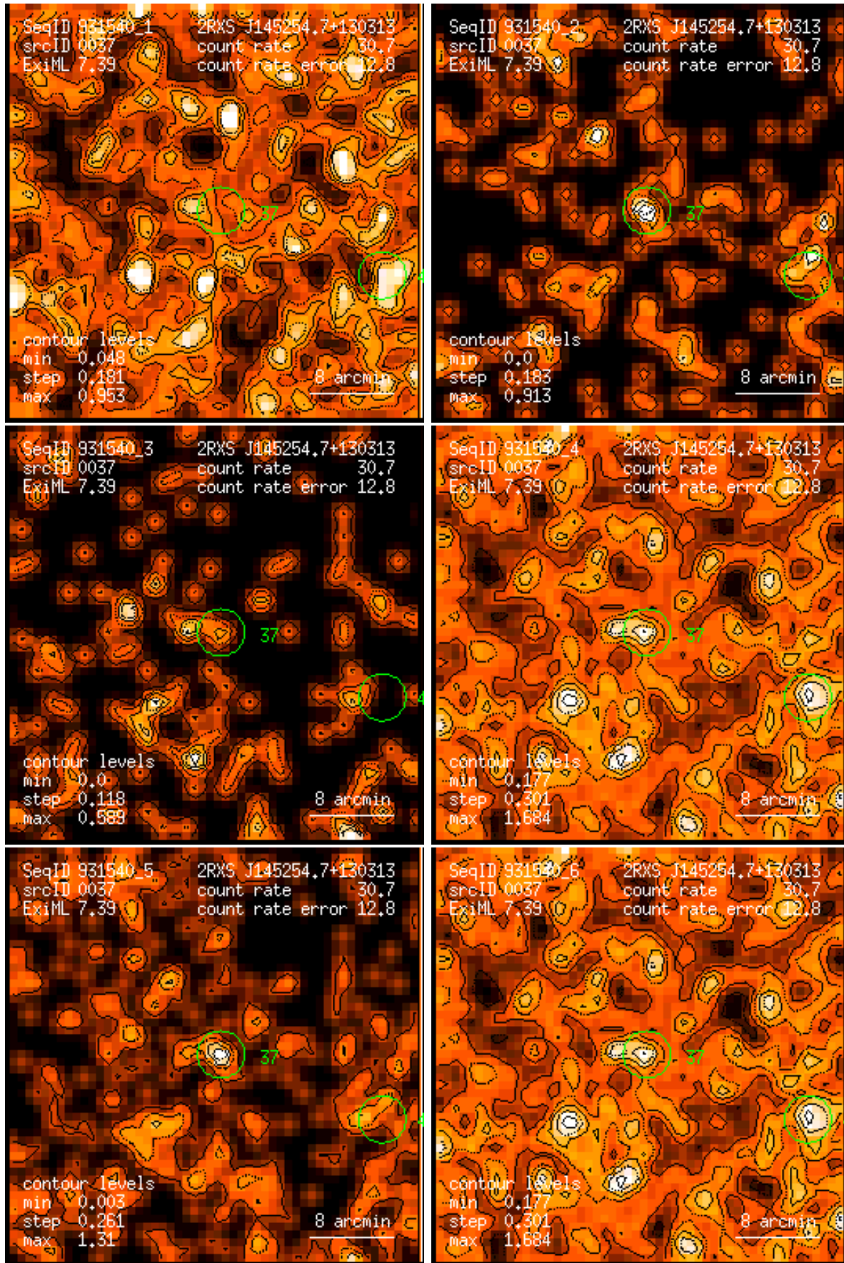
Figure 37: RASS 931540: detection 0037: band rate images, Gaussian filter: (1) PSPC channels 11 – 41, (2) 52 – 90, (3) 91 – 201, (4) 11 – 235, (5) 52 – 201, (6) 11 – 201. Broad band rates in counts/ks. Band rate contour levels in counts/ks/arcmin 2 .
