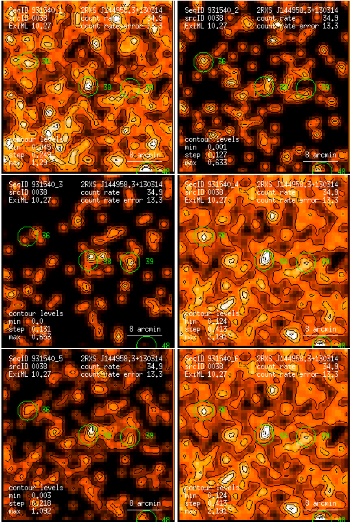
Figure 38: RASS 931540: detection 0038: band rate images, Gaussian filter: (1) PSPC channels 11 – 41, (2) 52 – 90, (3) 91 – 201, (4) 11 – 235, (5) 52 – 201, (6) 11 – 201. Broad band rates in counts/ks. Band rate contour levels in counts/ks/arcmin 2 .
