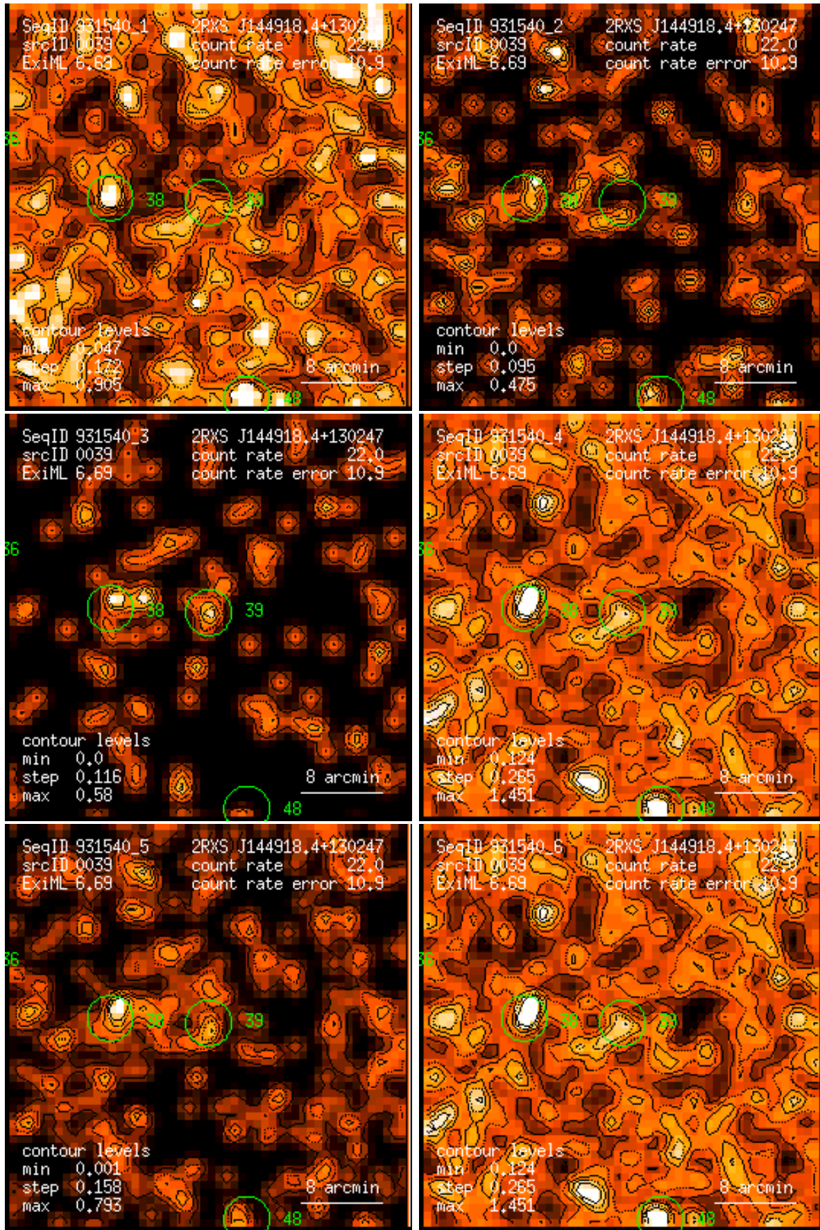
Figure 39: RASS 931540: detection 0039: band rate images, Gaussian filter: (1) PSPC channels 11 – 41, (2) 52 – 90, (3) 91 – 201, (4) 11 – 235, (5) 52 – 201, (6) 11 – 201. Broad band rates in counts/ks. Band rate contour levels in counts/ks/arcmin 2 .
