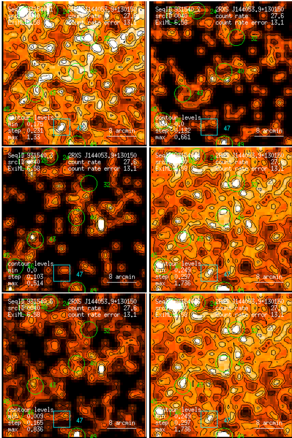
Figure 40: RASS 931540: detection 0040: band rate images, Gaussian filter: (1) PSPC channels 11 – 41, (2) 52 – 90, (3) 91 – 201, (4) 11 – 235, (5) 52 – 201, (6) 11 – 201. Broad band rates in counts/ks. Band rate contour levels in counts/ks/arcmin 2 .
