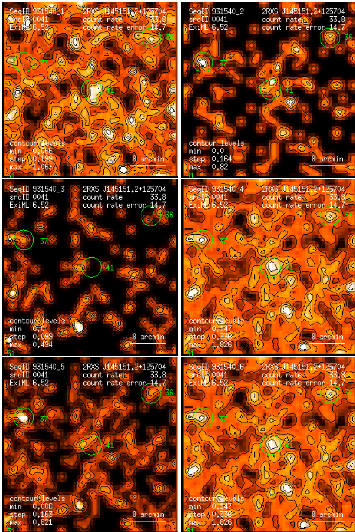
Figure 41: RASS 931540: detection 0041: band rate images, Gaussian filter: (1) PSPC channels 11 – 41, (2) 52 – 90, (3) 91 – 201, (4) 11 – 235, (5) 52 – 201, (6) 11 – 201. Broad band rates in counts/ks. Band rate contour levels in counts/ks/arcmin 2 .
