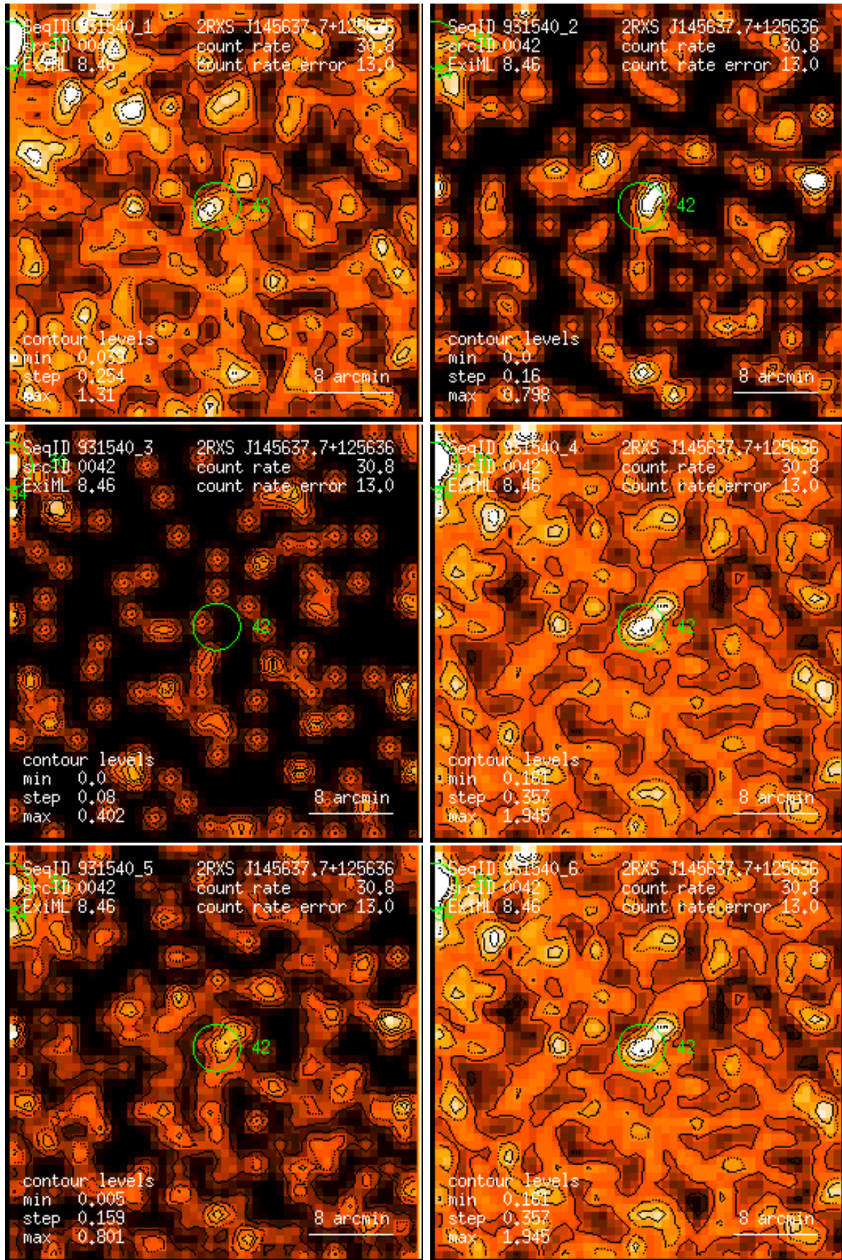
Figure 42: RASS 931540: detection 0042: band rate images, Gaussian filter: (1) PSPC channels 11 – 41, (2) 52 – 90, (3) 91 – 201, (4) 11 – 235, (5) 52 – 201, (6) 11 – 201. Broad band rates in counts/ks. Band rate contour levels in counts/ks/arcmin 2 .
