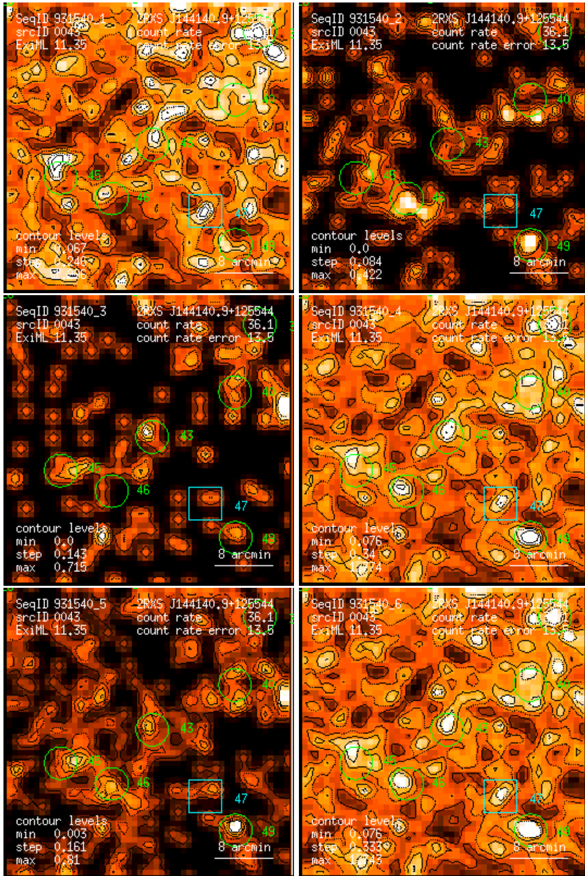
Figure 43: RASS 931540: detection 0043: band rate images, Gaussian filter: (1) PSPC channels 11 – 41, (2) 52 – 90, (3) 91 – 201, (4) 11 – 235, (5) 52 – 201, (6) 11 – 201. Broad band rates in counts/ks. Band rate contour levels in counts/ks/arcmin 2 .
