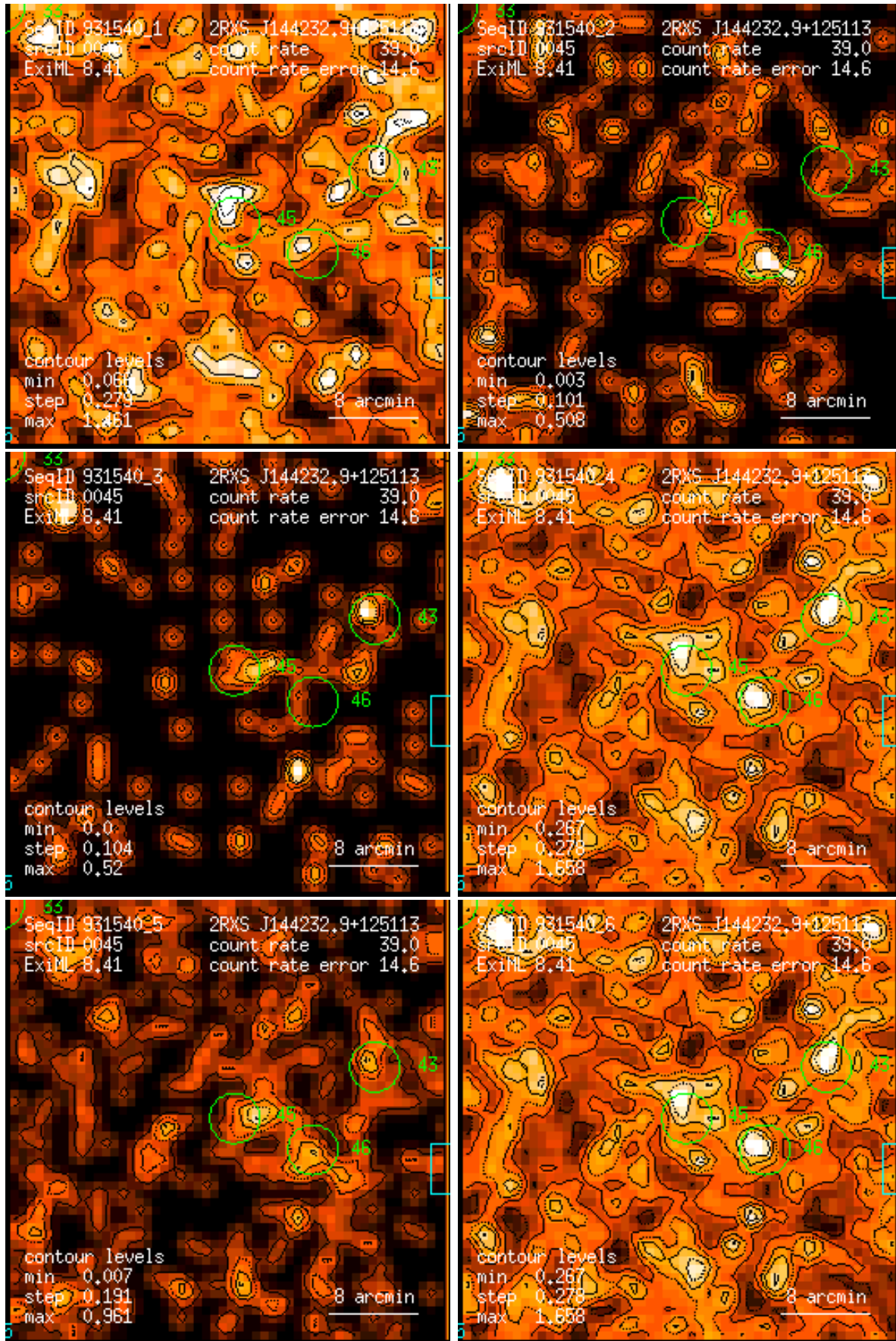
Figure 45: RASS 931540: detection 0045: band rate images, Gaussian filter: (1) PSPC channels 11 – 41, (2) 52 – 90, (3) 91 – 201, (4) 11 – 235, (5) 52 – 201, (6) 11 – 201. Broad band rates in counts/ks. Band rate contour levels in counts/ks/arcmin 2 .
