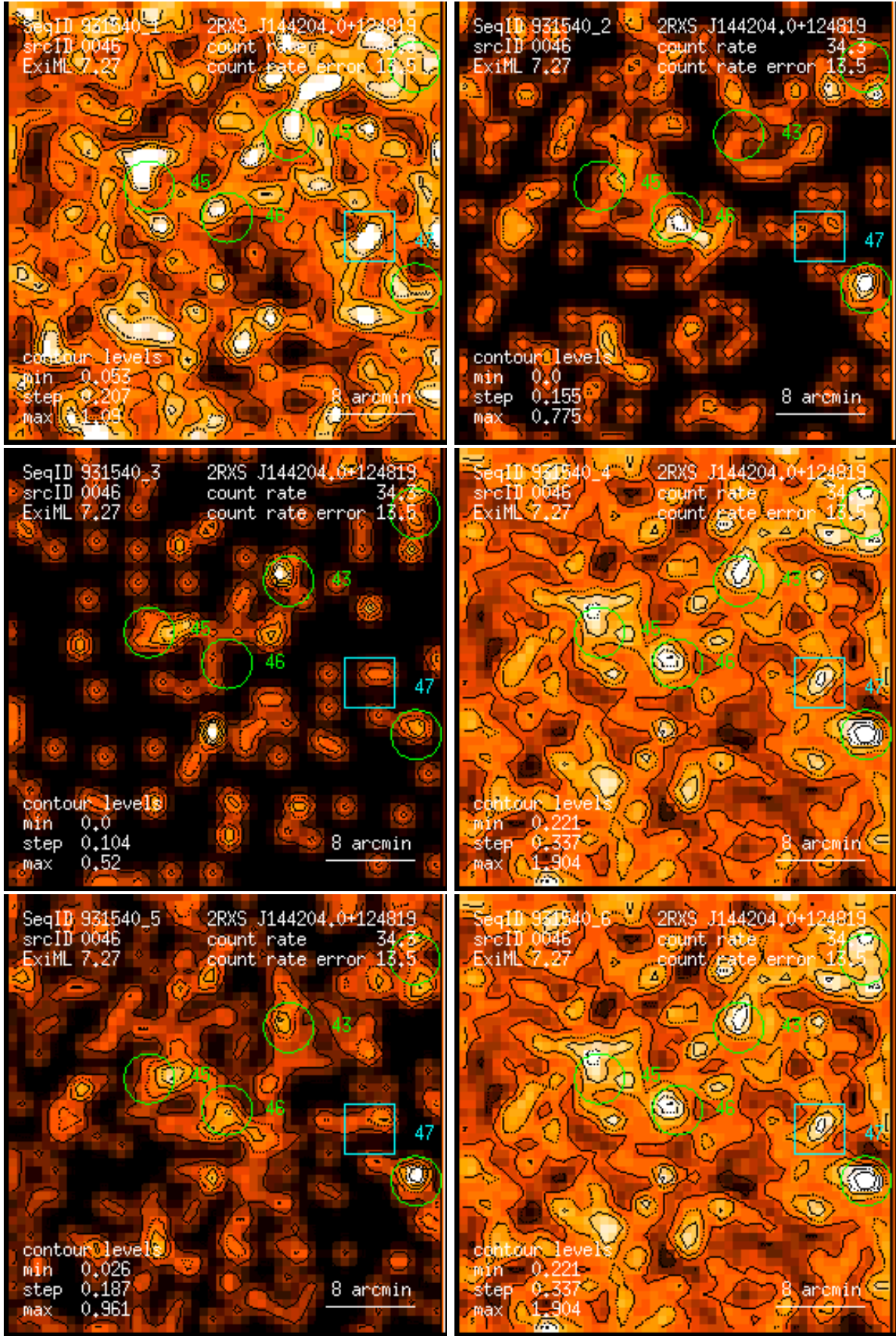
Figure 46: RASS 931540: detection 0046: band rate images, Gaussian filter: (1) PSPC channels 11 – 41, (2) 52 – 90, (3) 91 – 201, (4) 11 – 235, (5) 52 – 201, (6) 11 – 201. Broad band rates in counts/ks. Band rate contour levels in counts/ks/arcmin 2 .
