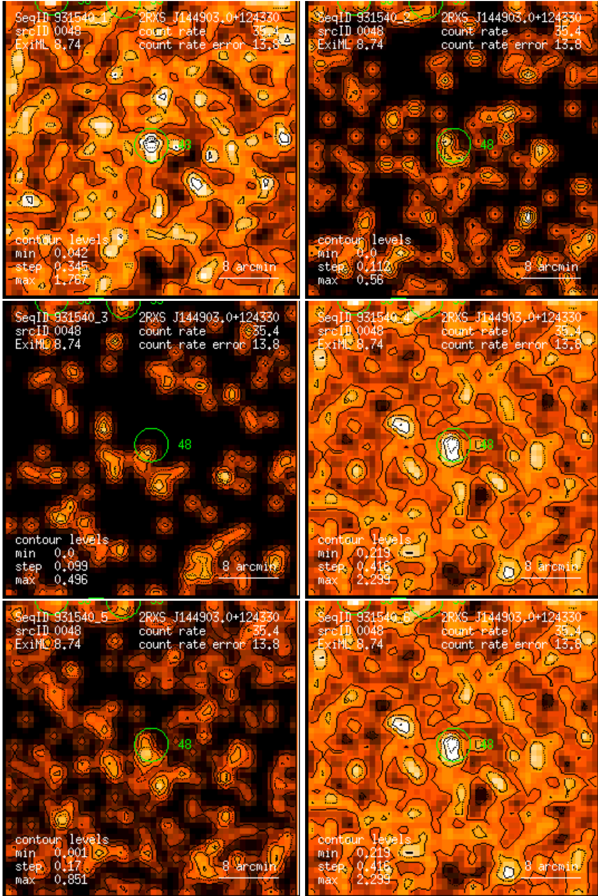
Figure 48: RASS 931540: detection 0048: band rate images, Gaussian filter: (1) PSPC channels 11 – 41, (2) 52 – 90, (3) 91 – 201, (4) 11 – 235, (5) 52 – 201, (6) 11 – 201. Broad band rates in counts/ks. Band rate contour levels in counts/ks/arcmin 2 .
