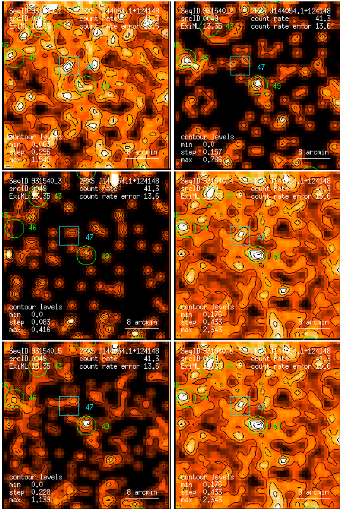
Figure 49: RASS 931540: detection 0049: band rate images, Gaussian filter: (1) PSPC channels 11 – 41, (2) 52 – 90, (3) 91 – 201, (4) 11 – 235, (5) 52 – 201, (6) 11 – 201. Broad band rates in counts/ks. Band rate contour levels in counts/ks/arcmin 2 .
