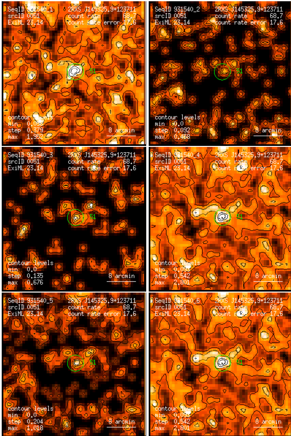
Figure 51: RASS 931540: detection 0051: band rate images, Gaussian filter: (1) PSPC channels 11 – 41, (2) 52 – 90, (3) 91 – 201, (4) 11 – 235, (5) 52 – 201, (6) 11 – 201. Broad band rates in counts/ks. Band rate contour levels in counts/ks/arcmin 2 .
