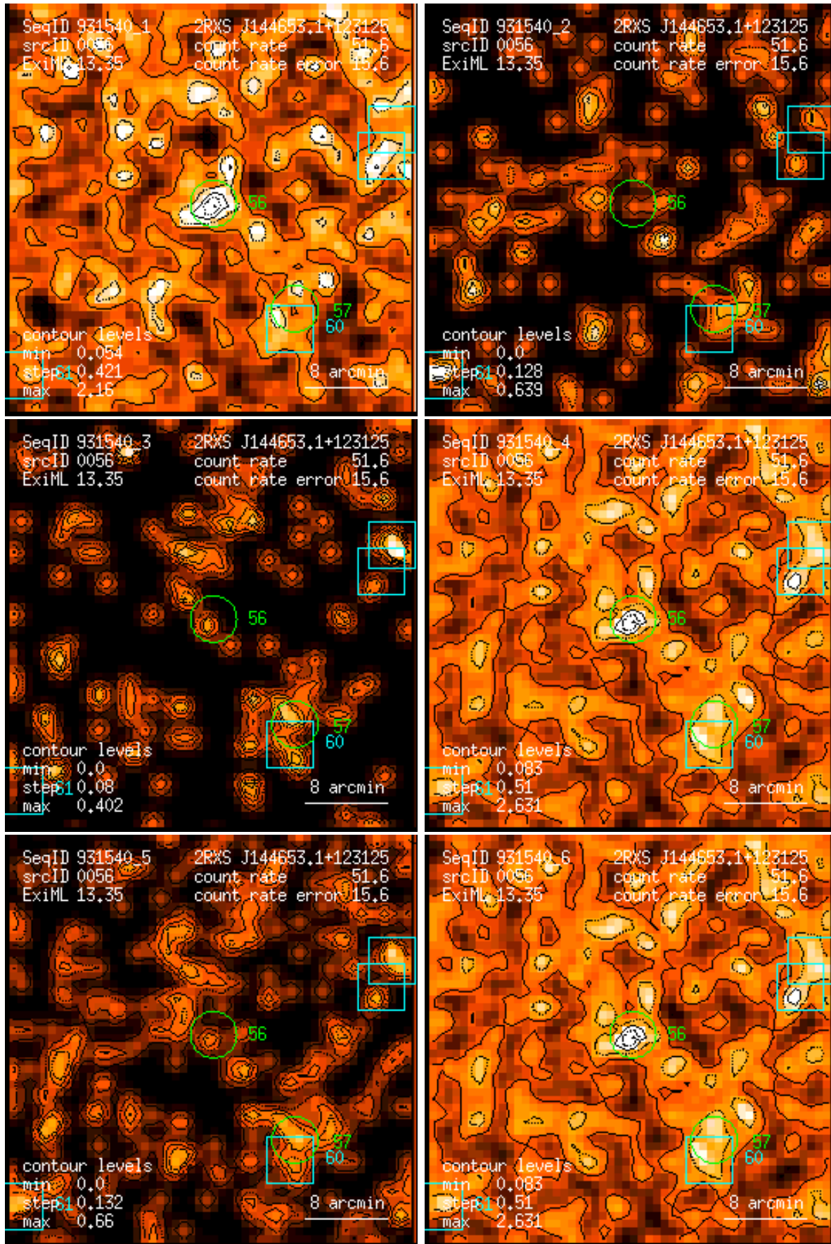
Figure 56: RASS 931540: detection 0056: band rate images, Gaussian filter: (1) PSPC channels 11 – 41, (2) 52 – 90, (3) 91 – 201, (4) 11 – 235, (5) 52 – 201, (6) 11 – 201. Broad band rates in counts/ks. Band rate contour levels in counts/ks/arcmin 2 .
