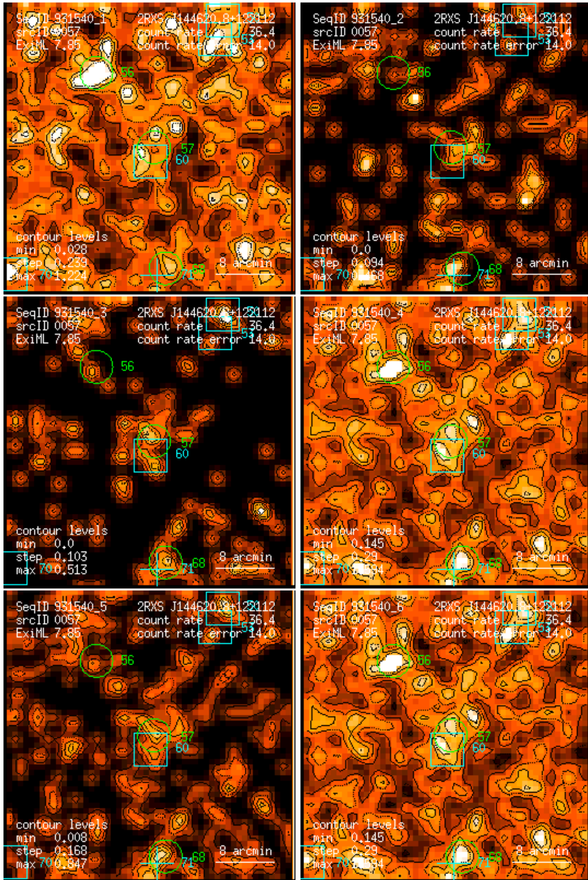
Figure 57: RASS 931540: detection 0057: band rate images, Gaussian filter: (1) PSPC channels 11 – 41, (2) 52 – 90, (3) 91 – 201, (4) 11 – 235, (5) 52 – 201, (6) 11 – 201. Broad band rates in counts/ks. Band rate contour levels in counts/ks/arcmin 2 .
