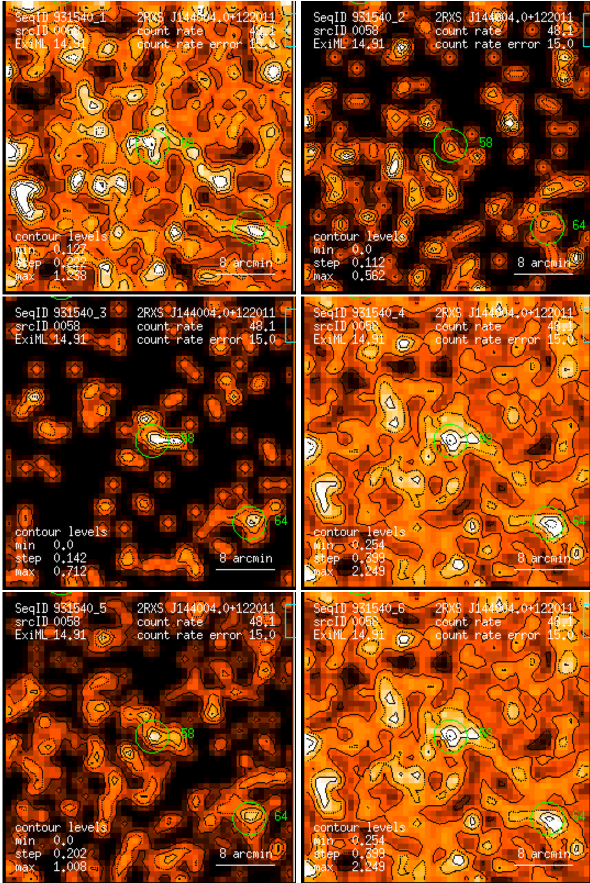
Figure 58: RASS 931540: detection 0058: band rate images, Gaussian filter: (1) PSPC channels 11 – 41, (2) 52 – 90, (3) 91 – 201, (4) 11 – 235, (5) 52 – 201, (6) 11 – 201. Broad band rates in counts/ks. Band rate contour levels in counts/ks/arcmin 2 .
