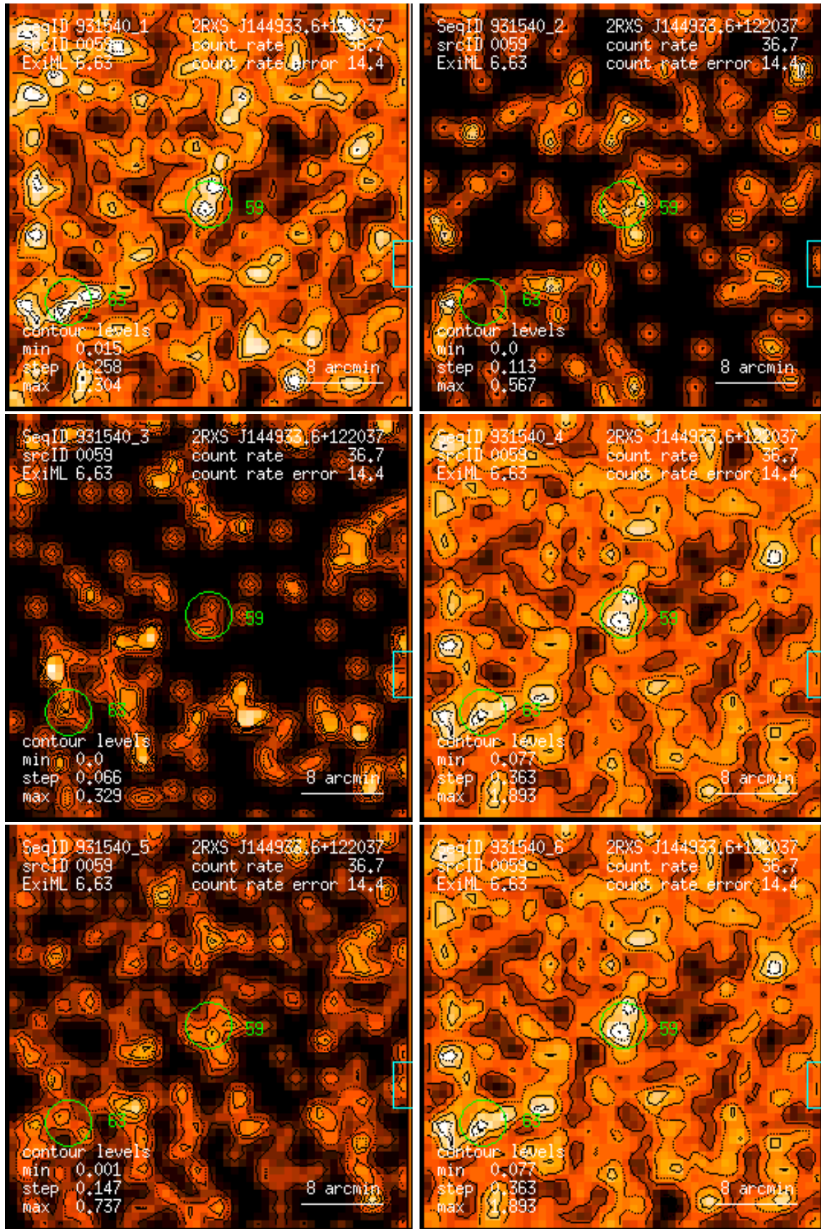
Figure 59: RASS 931540: detection 0059: band rate images, Gaussian filter: (1) PSPC channels 11 – 41, (2) 52 – 90, (3) 91 – 201, (4) 11 – 235, (5) 52 – 201, (6) 11 – 201. Broad band rates in counts/ks. Band rate contour levels in counts/ks/arcmin 2 .
