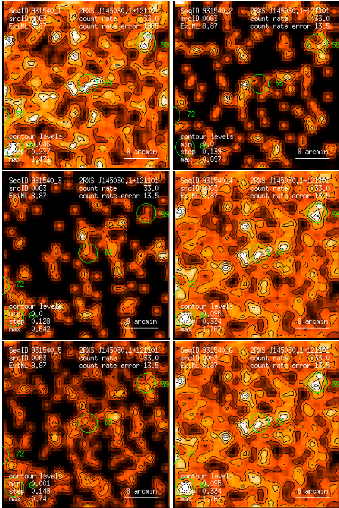
Figure 63: RASS 931540: detection 0063: band rate images, Gaussian filter: (1) PSPC channels 11 – 41, (2) 52 – 90, (3) 91 – 201, (4) 11 – 235, (5) 52 – 201, (6) 11 – 201. Broad band rates in counts/ks. Band rate contour levels in counts/ks/arcmin 2 .
