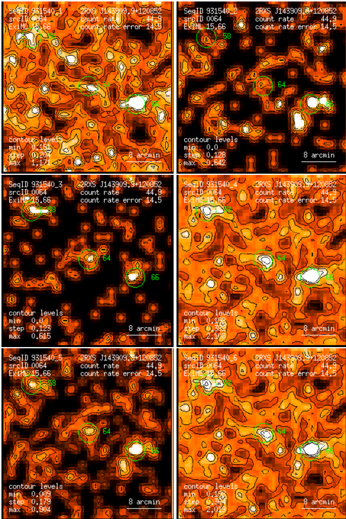
Figure 64: RASS 931540: detection 0064: band rate images, Gaussian filter: (1) PSPC channels 11 – 41, (2) 52 – 90, (3) 91 – 201, (4) 11 – 235, (5) 52 – 201, (6) 11 – 201. Broad band rates in counts/ks. Band rate contour levels in counts/ks/arcmin 2 .
