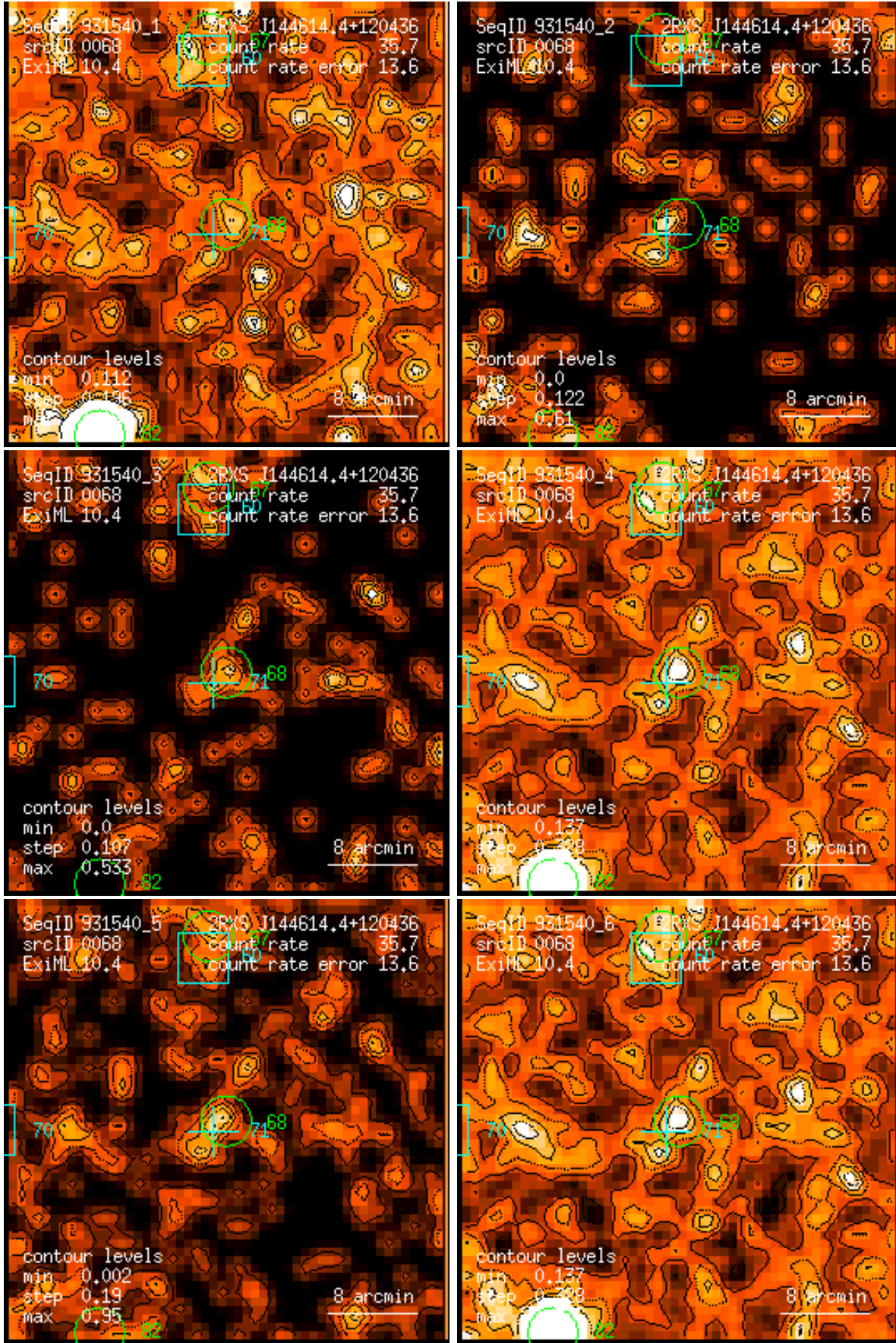
Figure 68: RASS 931540: detection 0068: band rate images, Gaussian filter: (1) PSPC channels 11 – 41, (2) 52 – 90, (3) 91 – 201, (4) 11 – 235, (5) 52 – 201, (6) 11 – 201. Broad band rates in counts/ks. Band rate contour levels in counts/ks/arcmin 2 .
