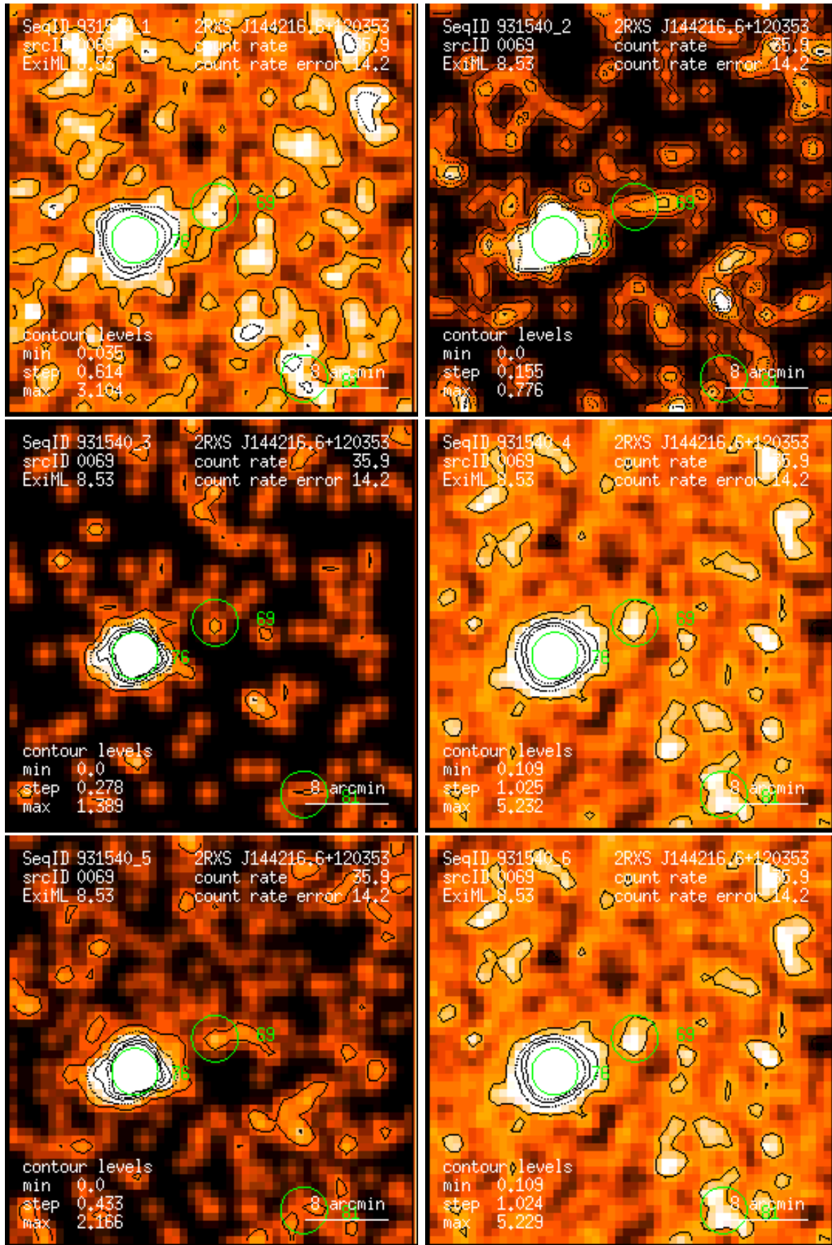
Figure 69: RASS 931540: detection 0069: band rate images, Gaussian filter: (1) PSPC channels 11 – 41, (2) 52 – 90, (3) 91 – 201, (4) 11 – 235, (5) 52 – 201, (6) 11 – 201. Broad band rates in counts/ks. Band rate contour levels in counts/ks/arcmin 2 .
