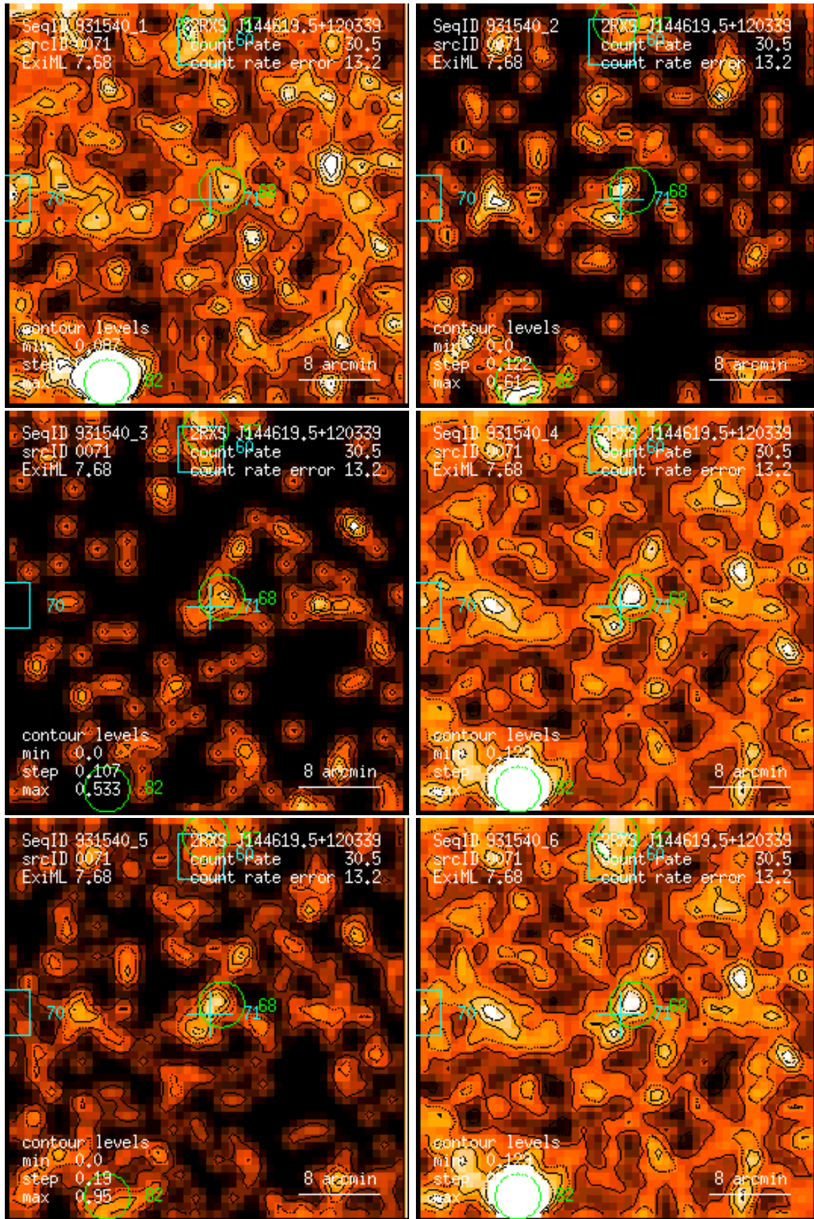
Figure 71: RASS 931540: detection 0071: band rate images, Gaussian filter: (1) PSPC channels 11 – 41, (2) 52 – 90, (3) 91 – 201, (4) 11 – 235, (5) 52 – 201, (6) 11 – 201. Broad band rates in counts/ks. Band rate contour levels in counts/ks/arcmin 2 .
