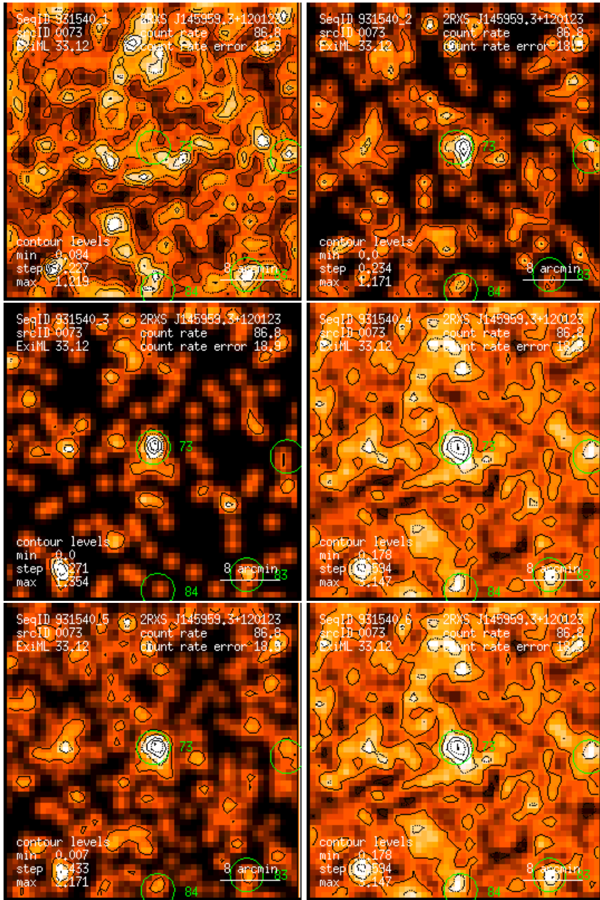
Figure 73: RASS 931540: detection 0073: band rate images, Gaussian filter: (1) PSPC channels 11 – 41, (2) 52 – 90, (3) 91 – 201, (4) 11 – 235, (5) 52 – 201, (6) 11 – 201. Broad band rates in counts/ks. Band rate contour levels in counts/ks/arcmin 2 .
