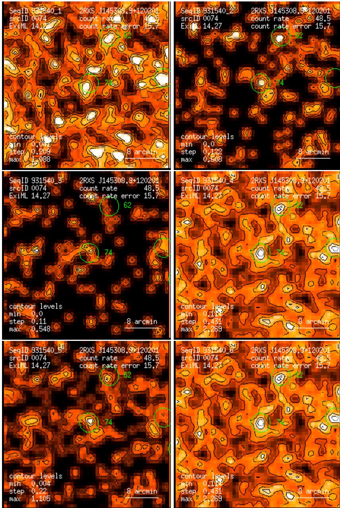
Figure 74: RASS 931540: detection 0074: band rate images, Gaussian filter: (1) PSPC channels 11 – 41, (2) 52 – 90, (3) 91 – 201, (4) 11 – 235, (5) 52 – 201, (6) 11 – 201. Broad band rates in counts/ks. Band rate contour levels in counts/ks/arcmin 2 .
