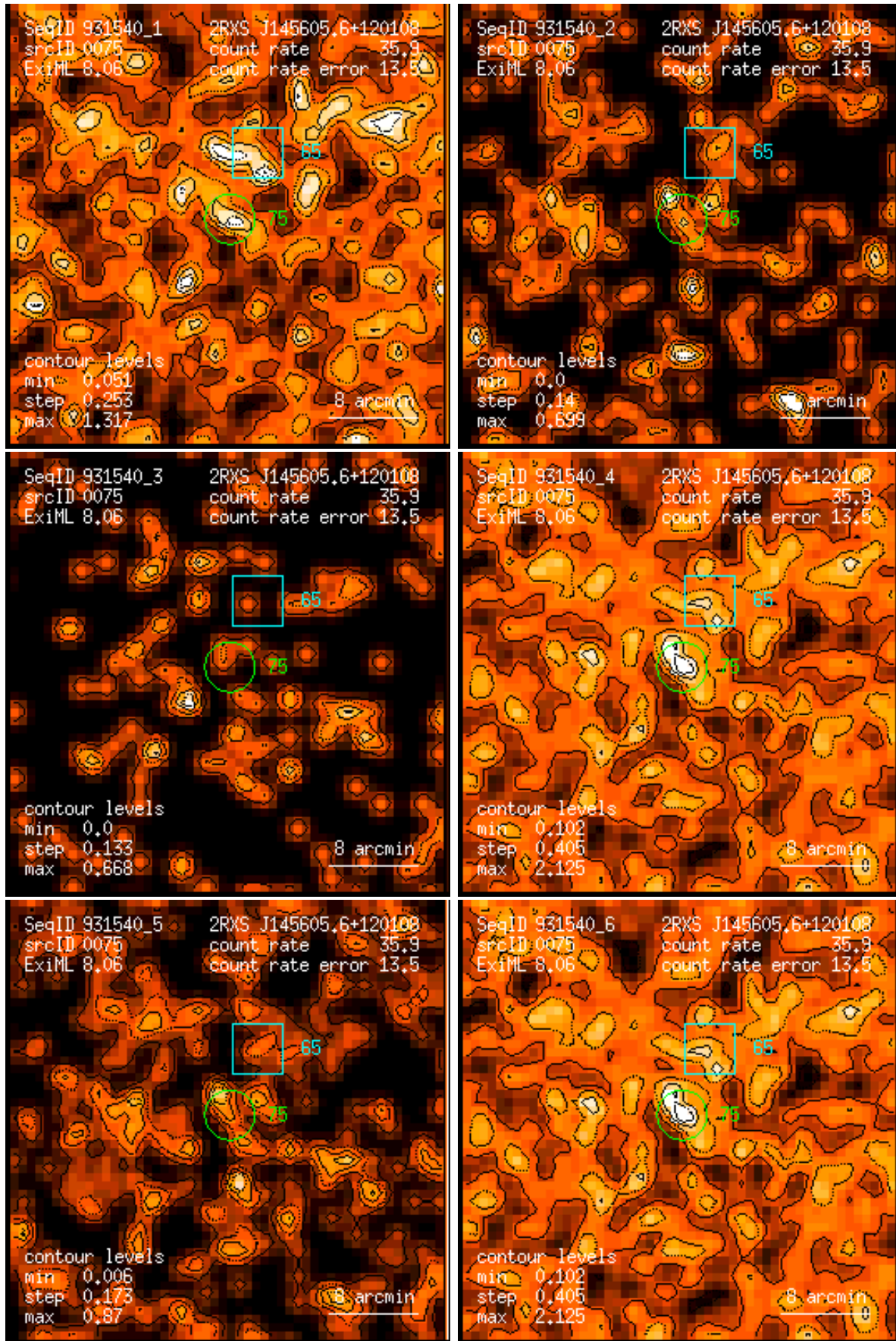
Figure 75: RASS 931540: detection 0075: band rate images, Gaussian filter: (1) PSPC channels 11 – 41, (2) 52 – 90, (3) 91 – 201, (4) 11 – 235, (5) 52 – 201, (6) 11 – 201. Broad band rates in counts/ks. Band rate contour levels in counts/ks/arcmin 2 .
