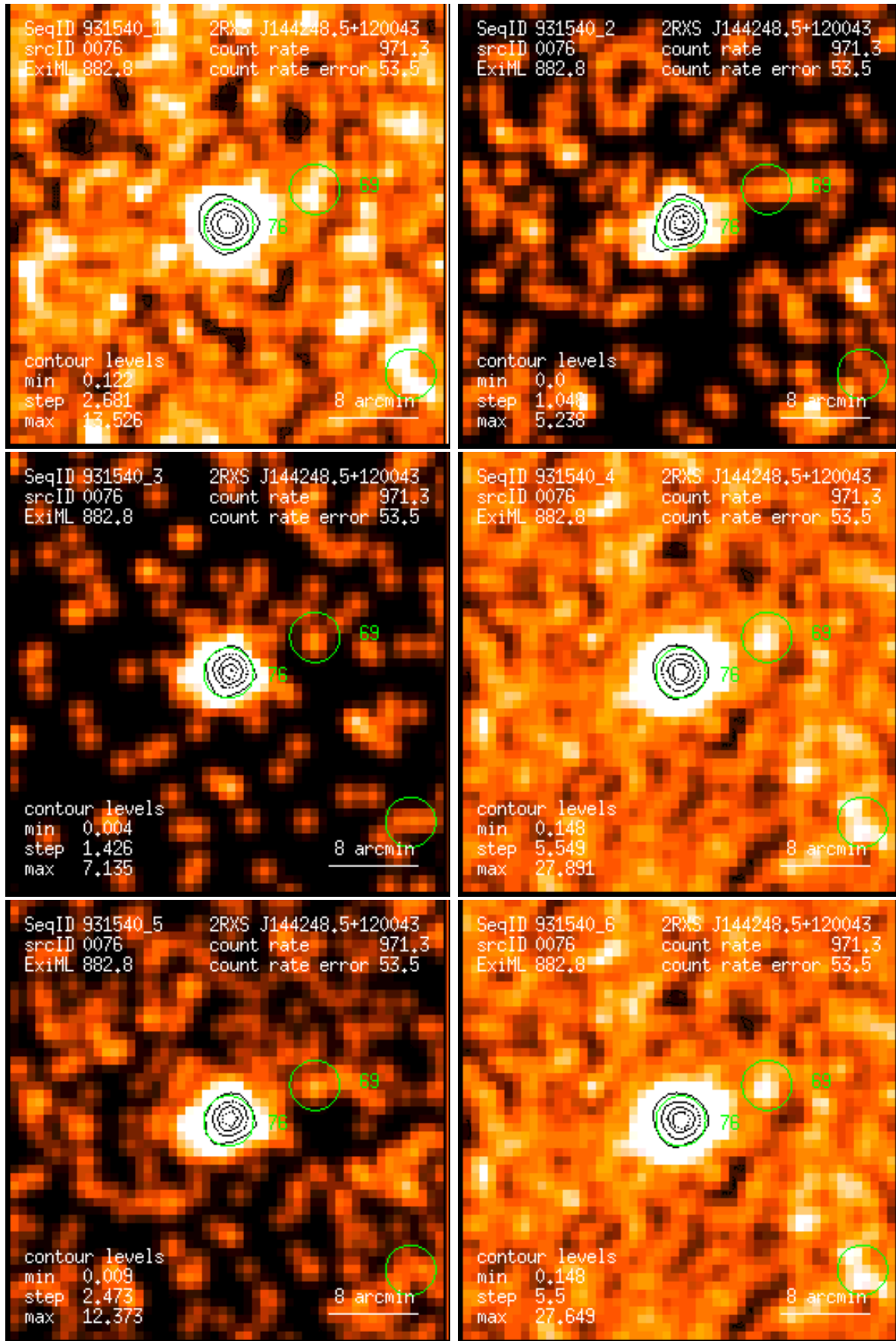
Figure 76: RASS 931540: detection 0076: band rate images, Gaussian filter: (1) PSPC channels 11 – 41, (2) 52 – 90, (3) 91 – 201, (4) 11 – 235, (5) 52 – 201, (6) 11 – 201. Broad band rates in counts/ks. Band rate contour levels in counts/ks/arcmin 2 .
