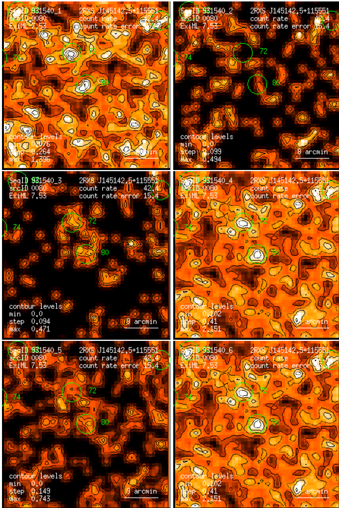
Figure 80: RASS 931540: detection 0080: band rate images, Gaussian filter: (1) PSPC channels 11 – 41, (2) 52 – 90, (3) 91 – 201, (4) 11 – 235, (5) 52 – 201, (6) 11 – 201. Broad band rates in counts/ks. Band rate contour levels in counts/ks/arcmin 2 .
