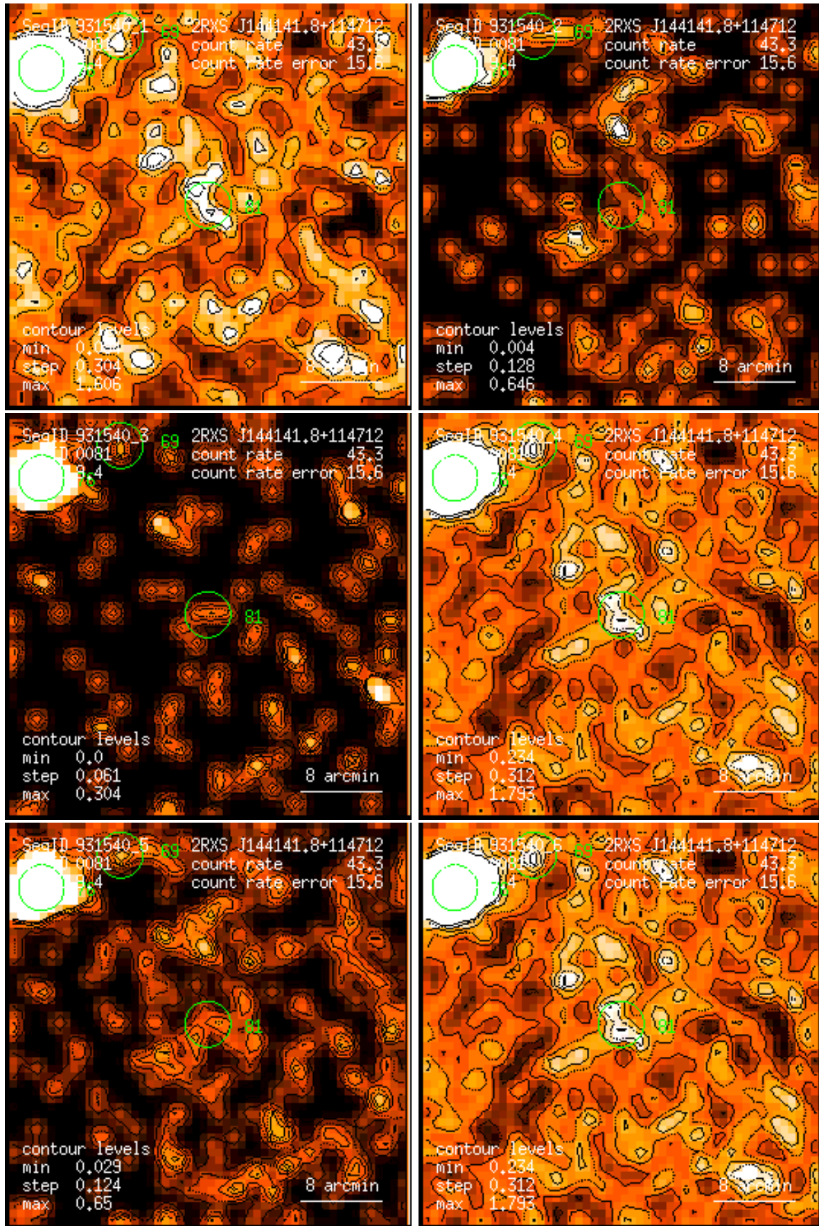
Figure 81: RASS 931540: detection 0081: band rate images, Gaussian filter: (1) PSPC channels 11 – 41, (2) 52 – 90, (3) 91 – 201, (4) 11 – 235, (5) 52 – 201, (6) 11 – 201. Broad band rates in counts/ks. Band rate contour levels in counts/ks/arcmin 2 .
