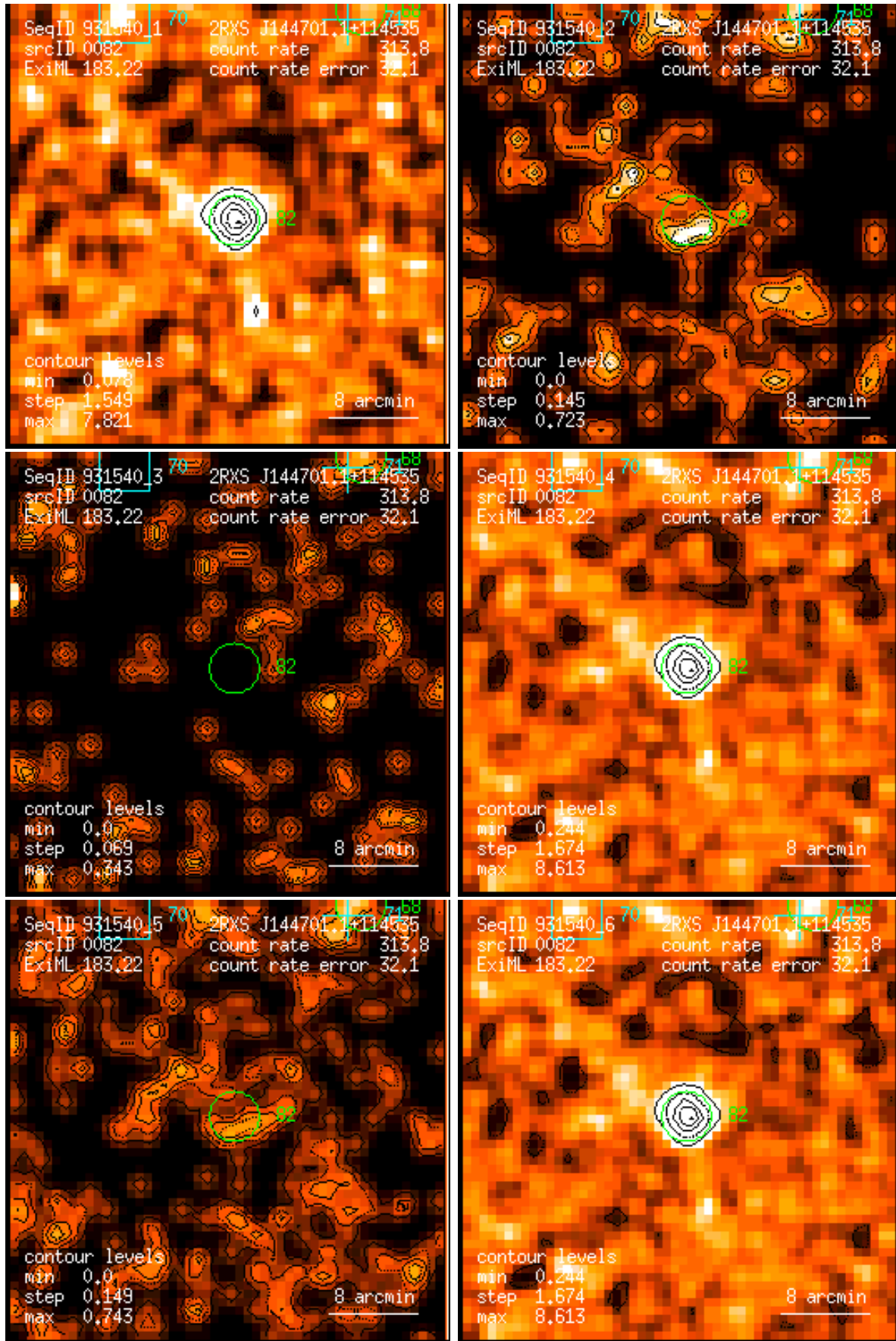
Figure 82: RASS 931540: detection 0082: band rate images, Gaussian filter: (1) PSPC channels 11 – 41, (2) 52 – 90, (3) 91 – 201, (4) 11 – 235, (5) 52 – 201, (6) 11 – 201. Broad band rates in counts/ks. Band rate contour levels in counts/ks/arcmin 2 .
