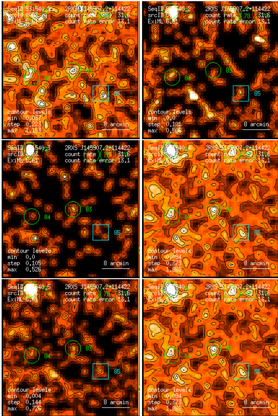
Figure 83: RASS 931540: detection 0083: band rate images, Gaussian filter: (1) PSPC channels 11 – 41, (2) 52 – 90, (3) 91 – 201, (4) 11 – 235, (5) 52 – 201, (6) 11 – 201. Broad band rates in counts/ks. Band rate contour levels in counts/ks/arcmin 2 .
