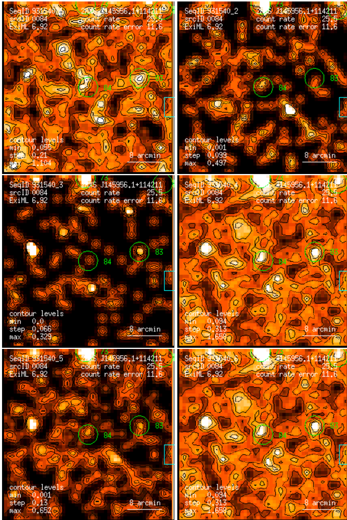
Figure 84: RASS 931540: detection 0084: band rate images, Gaussian filter: (1) PSPC channels 11 – 41, (2) 52 – 90, (3) 91 – 201, (4) 11 – 235, (5) 52 – 201, (6) 11 – 201. Broad band rates in counts/ks. Band rate contour levels in counts/ks/arcmin 2 .
