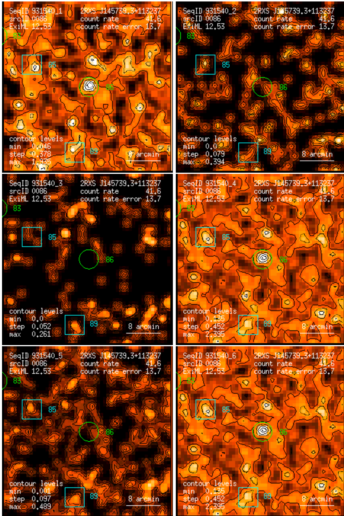
Figure 86: RASS 931540: detection 0086: band rate images, Gaussian filter: (1) PSPC channels 11 – 41, (2) 52 – 90, (3) 91 – 201, (4) 11 – 235, (5) 52 – 201, (6) 11 – 201. Broad band rates in counts/ks. Band rate contour levels in counts/ks/arcmin 2 .
