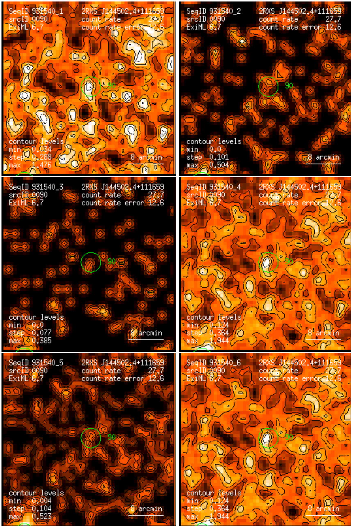
Figure 90: RASS 931540: detection 0090: band rate images, Gaussian filter: (1) PSPC channels 11 – 41, (2) 52 – 90, (3) 91 – 201, (4) 11 – 235, (5) 52 – 201, (6) 11 – 201. Broad band rates in counts/ks. Band rate contour levels in counts/ks/arcmin 2 .
