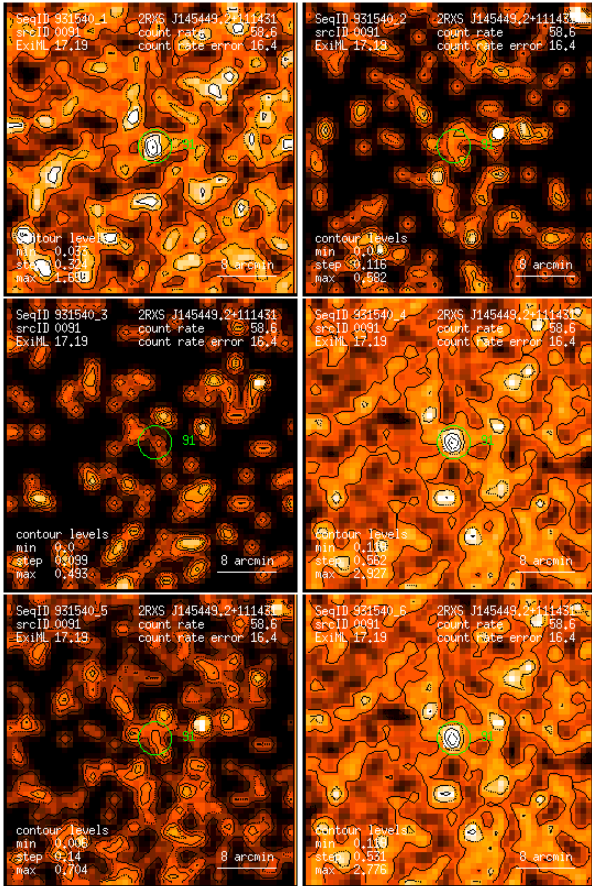
Figure 91: RASS 931540: detection 0091: band rate images, Gaussian filter: (1) PSPC channels 11 – 41, (2) 52 – 90, (3) 91 – 201, (4) 11 – 235, (5) 52 – 201, (6) 11 – 201. Broad band rates in counts/ks. Band rate contour levels in counts/ks/arcmin 2 .
