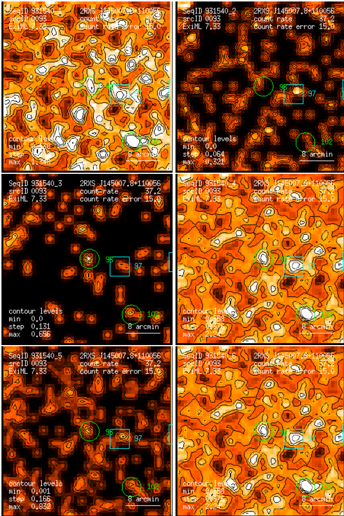
Figure 93: RASS 931540: detection 0093: band rate images, Gaussian filter: (1) PSPC channels 11 – 41, (2) 52 – 90, (3) 91 – 201, (4) 11 – 235, (5) 52 – 201, (6) 11 – 201. Broad band rates in counts/ks. Band rate contour levels in counts/ks/arcmin 2 .
