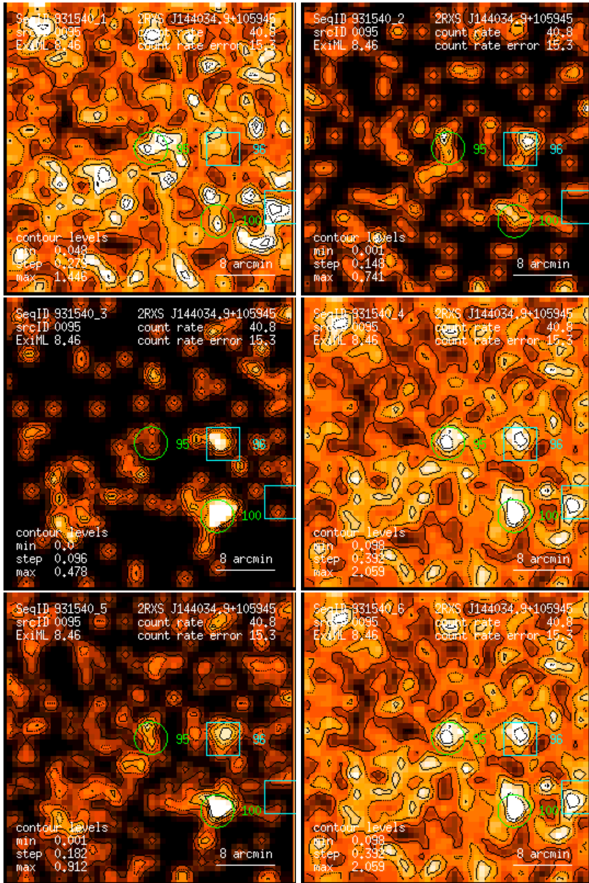
Figure 95: RASS 931540: detection 0095: band rate images, Gaussian filter: (1) PSPC channels 11 – 41, (2) 52 – 90, (3) 91 – 201, (4) 11 – 235, (5) 52 – 201, (6) 11 – 201. Broad band rates in counts/ks. Band rate contour levels in counts/ks/arcmin 2 .
