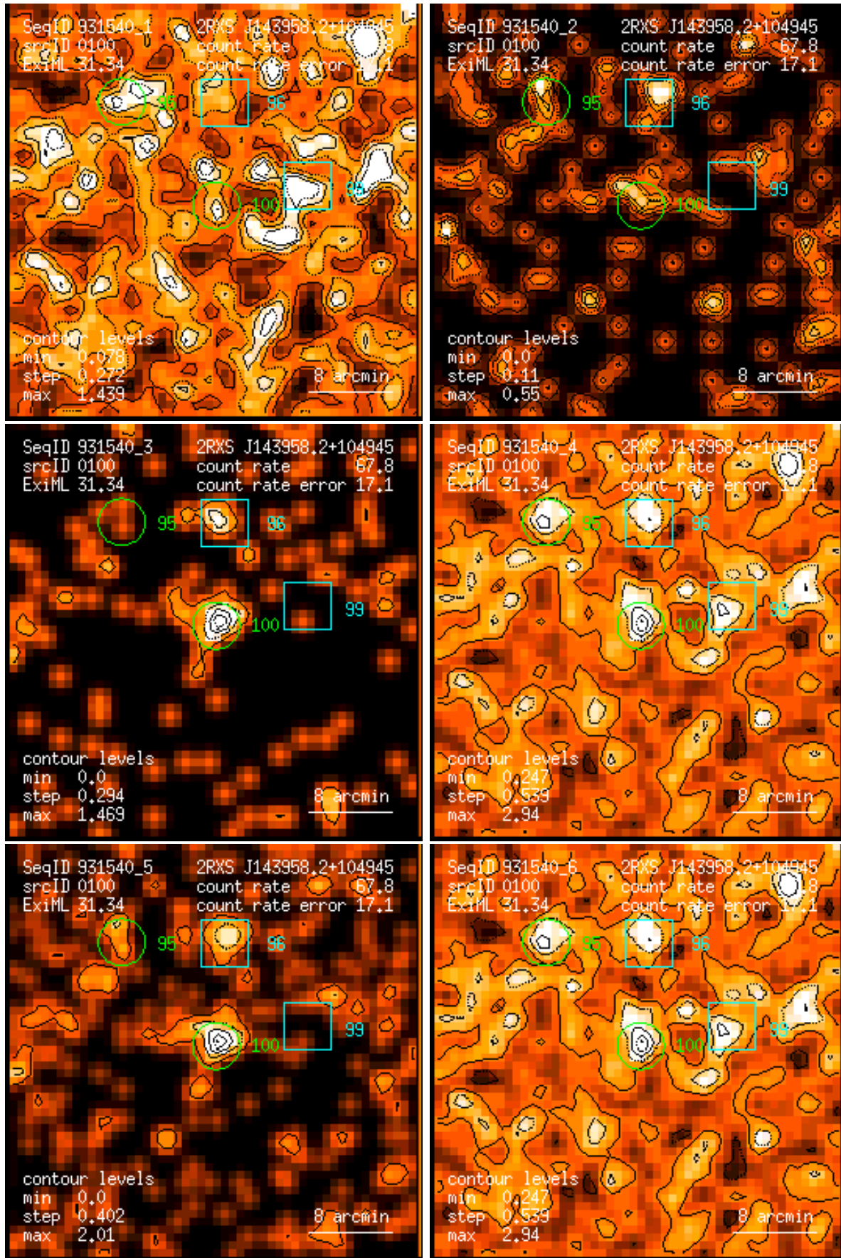
Figure 100: RASS 931540: detection 0100: band rate images, Gaussian filter: (1) PSPC channels 11 – 41, (2) 52 – 90, (3) 91 – 201, (4) 11 – 235, (5) 52 – 201, (6) 11 – 201. Broad band rates in counts/ks. Band rate contour levels in counts/ks/arcmin 2 .
