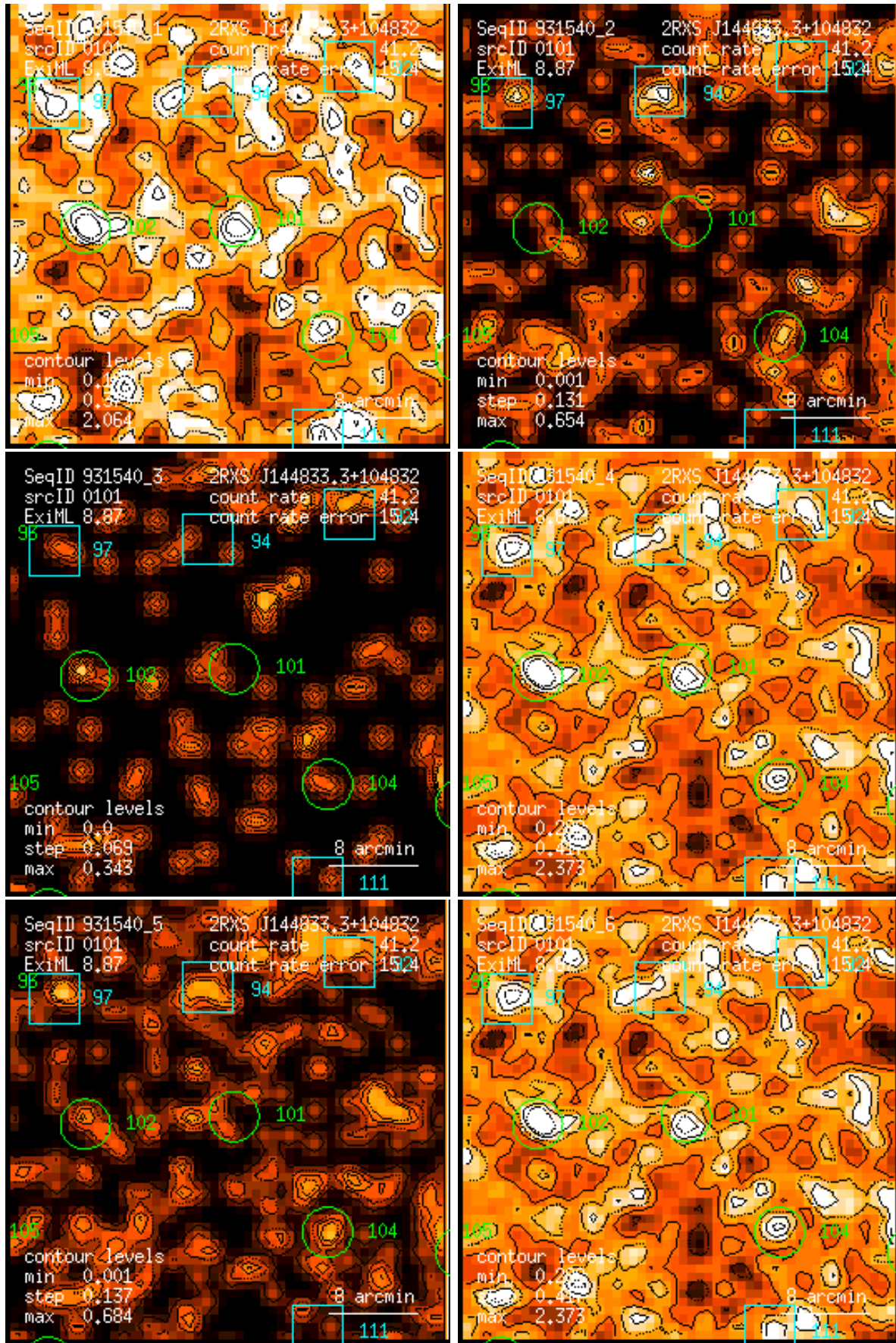
Figure 101: RASS 931540: detection 0101: band rate images, Gaussian filter: (1) PSPC channels 11 – 41, (2) 52 – 90, (3) 91 – 201, (4) 11 – 235, (5) 52 – 201, (6) 11 – 201. Broad band rates in counts/ks. Band rate contour levels in counts/ks/arcmin 2 .
