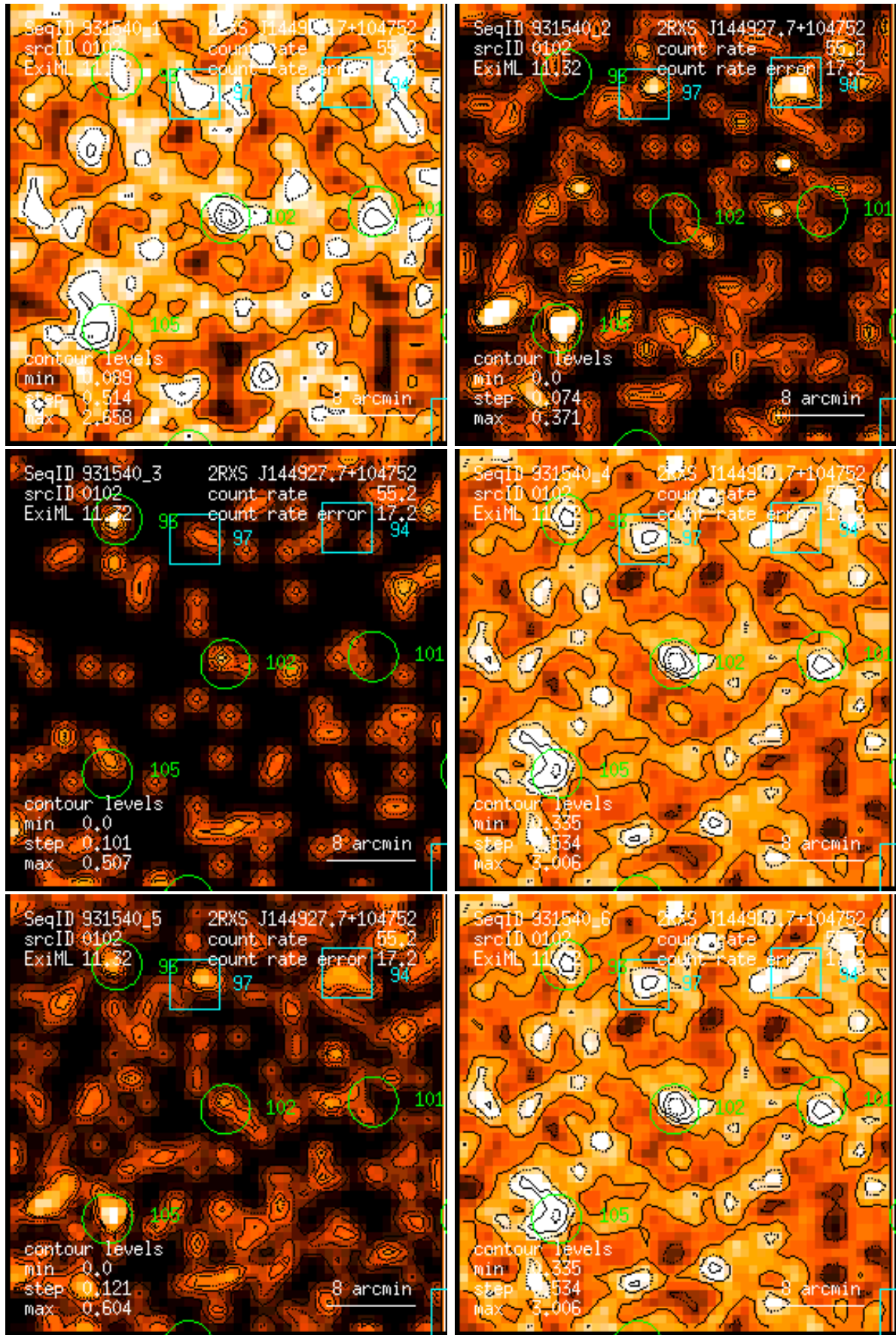
Figure 102: RASS 931540: detection 0102: band rate images, Gaussian filter: (1) PSPC channels 11 – 41, (2) 52 – 90, (3) 91 – 201, (4) 11 – 235, (5) 52 – 201, (6) 11 – 201. Broad band rates in counts/ks. Band rate contour levels in counts/ks/arcmin 2 .
