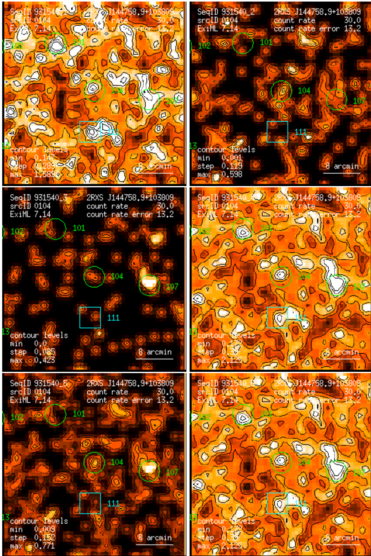
Figure 104: RASS 931540: detection 0104: band rate images, Gaussian filter: (1) PSPC channels 11 – 41, (2) 52 – 90, (3) 91 – 201, (4) 11 – 235, (5) 52 – 201, (6) 11 – 201. Broad band rates in counts/ks. Band rate contour levels in counts/ks/arcmin 2 .
