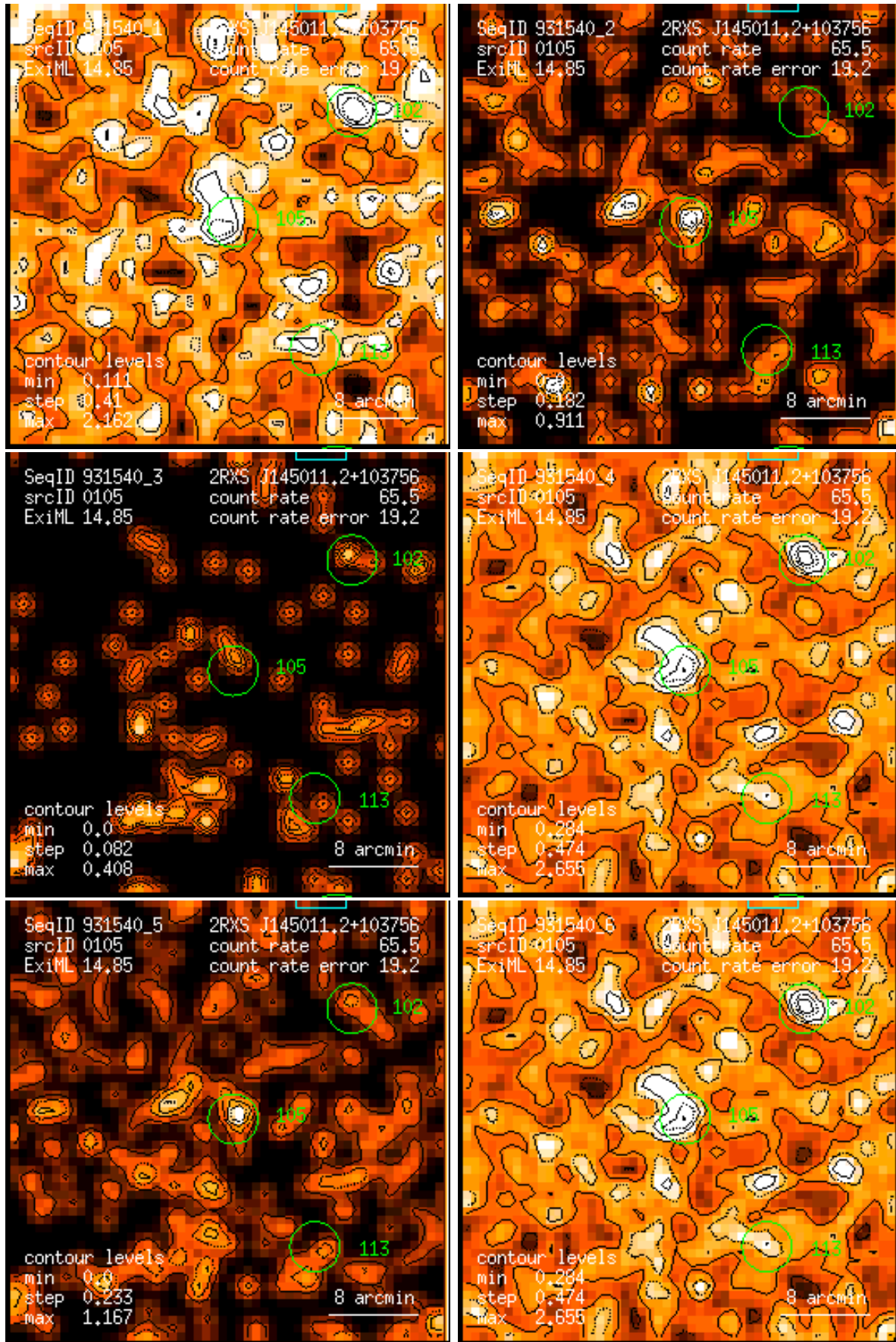
Figure 105: RASS 931540: detection 0105: band rate images, Gaussian filter: (1) PSPC channels 11 – 41, (2) 52 – 90, (3) 91 – 201, (4) 11 – 235, (5) 52 – 201, (6) 11 – 201. Broad band rates in counts/ks. Band rate contour levels in counts/ks/arcmin 2 .
