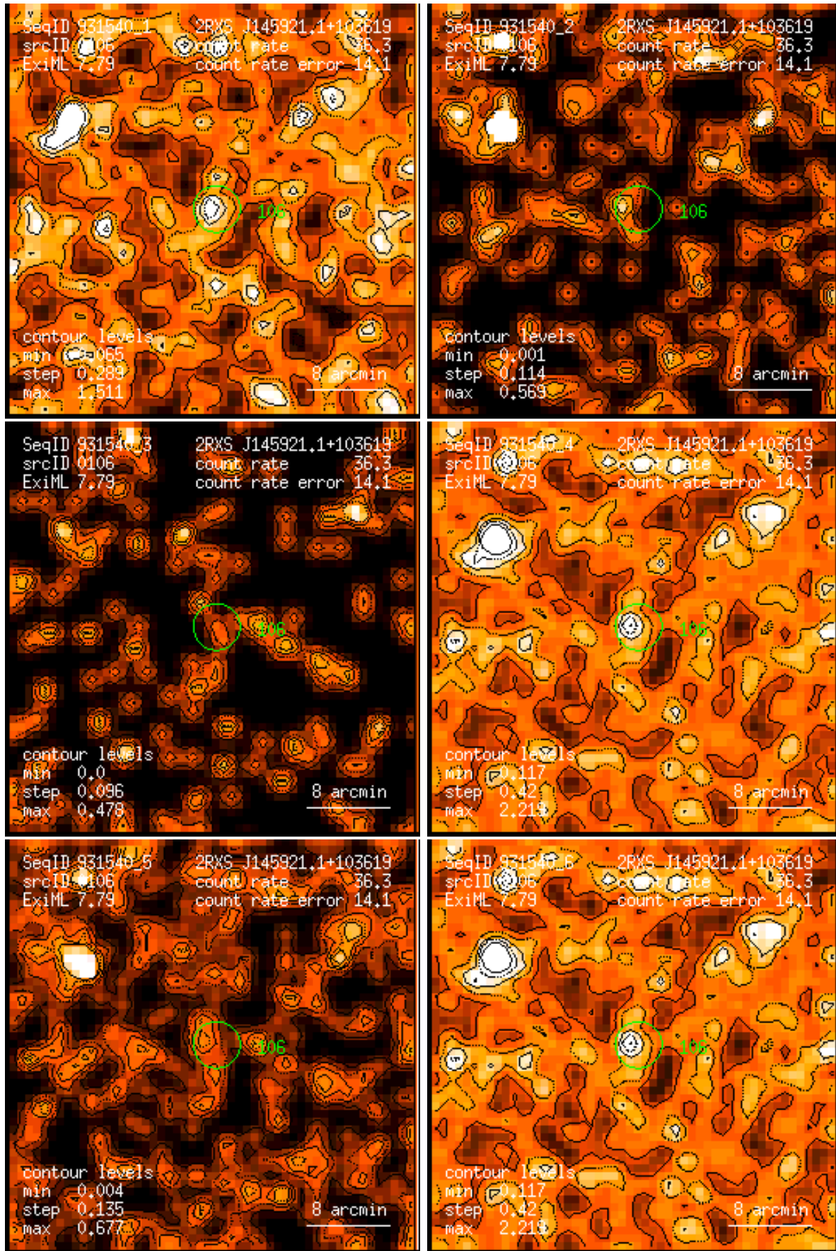
Figure 106: RASS 931540: detection 0106: band rate images, Gaussian filter: (1) PSPC channels 11 – 41, (2) 52 – 90, (3) 91 – 201, (4) 11 – 235, (5) 52 – 201, (6) 11 – 201. Broad band rates in counts/ks. Band rate contour levels in counts/ks/arcmin 2 .
