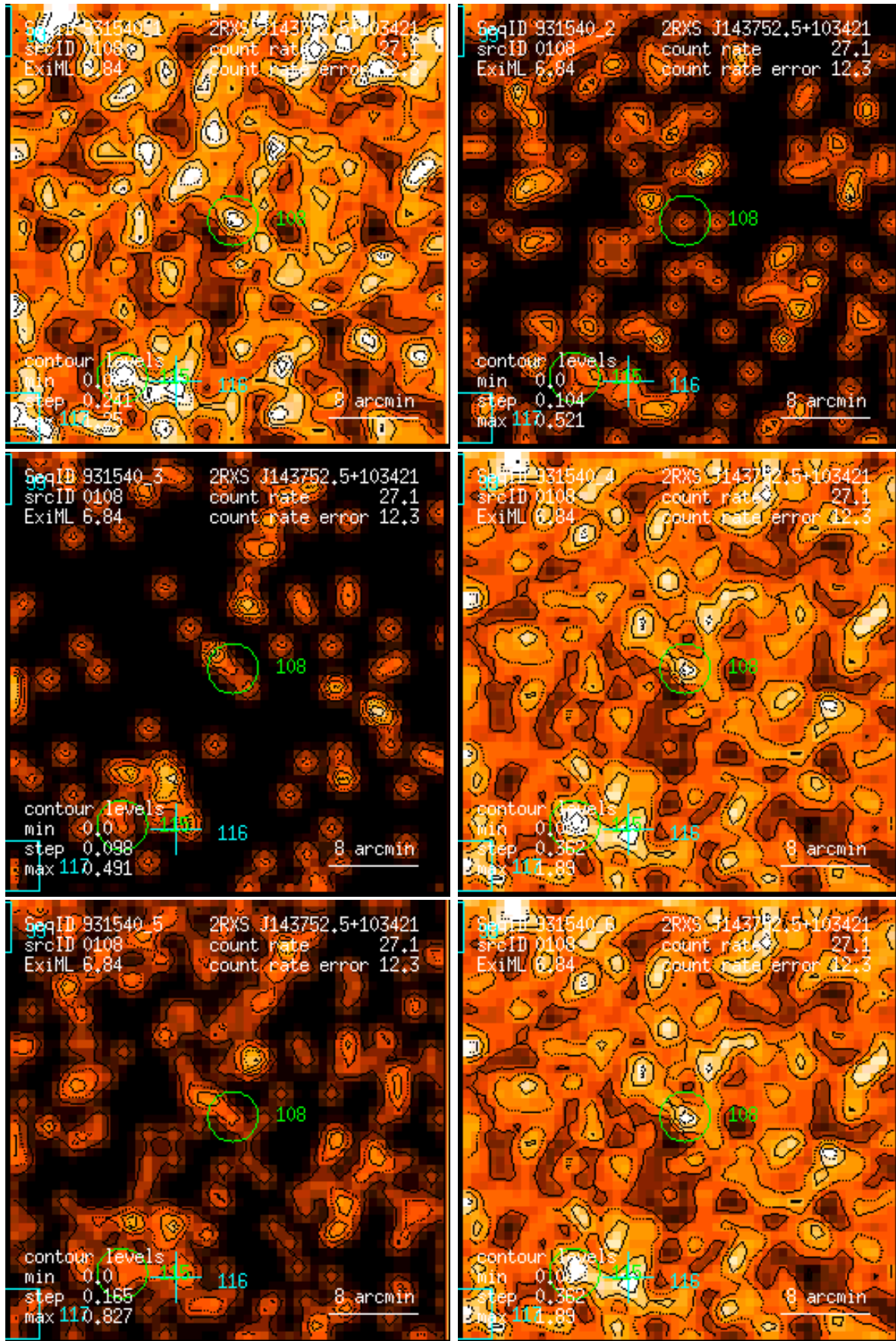
Figure 108: RASS 931540: detection 0108: band rate images, Gaussian filter: (1) PSPC channels 11 – 41, (2) 52 – 90, (3) 91 – 201, (4) 11 – 235, (5) 52 – 201, (6) 11 – 201. Broad band rates in counts/ks. Band rate contour levels in counts/ks/arcmin 2 .
