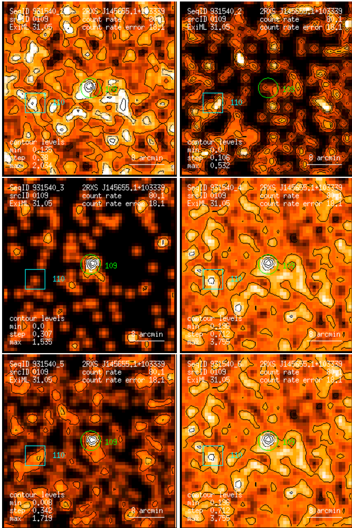
Figure 109: RASS 931540: detection 0109: band rate images, Gaussian filter: (1) PSPC channels 11 – 41, (2) 52 – 90, (3) 91 – 201, (4) 11 – 235, (5) 52 – 201, (6) 11 – 201. Broad band rates in counts/ks. Band rate contour levels in counts/ks/arcmin 2 .
