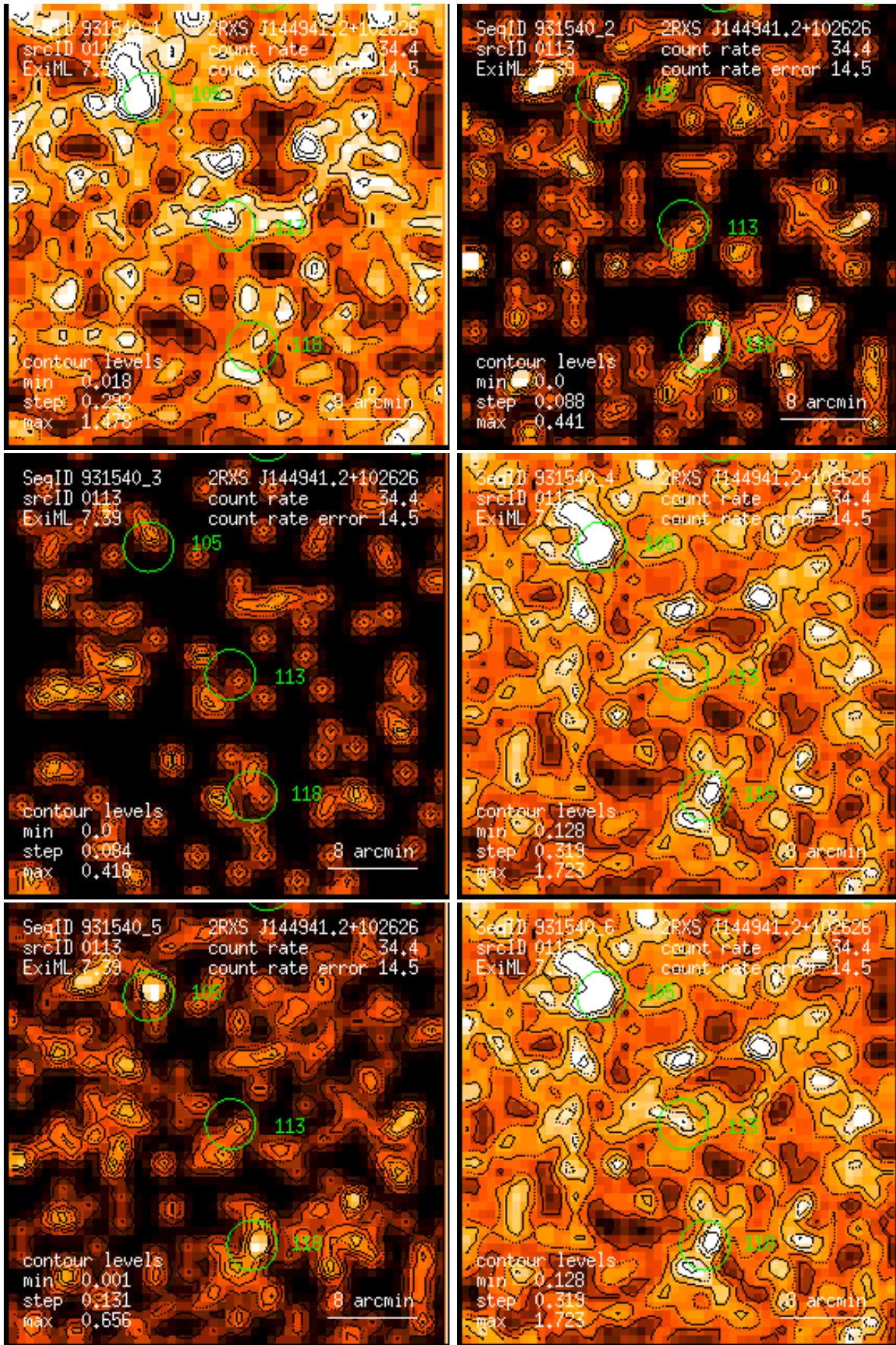
Figure 113: RASS 931540: detection 0113: band rate images, Gaussian filter: (1) PSPC channels 11 – 41, (2) 52 – 90, (3) 91 – 201, (4) 11 – 235, (5) 52 – 201, (6) 11 – 201. Broad band rates in counts/ks. Band rate contour levels in counts/ks/arcmin 2 .
