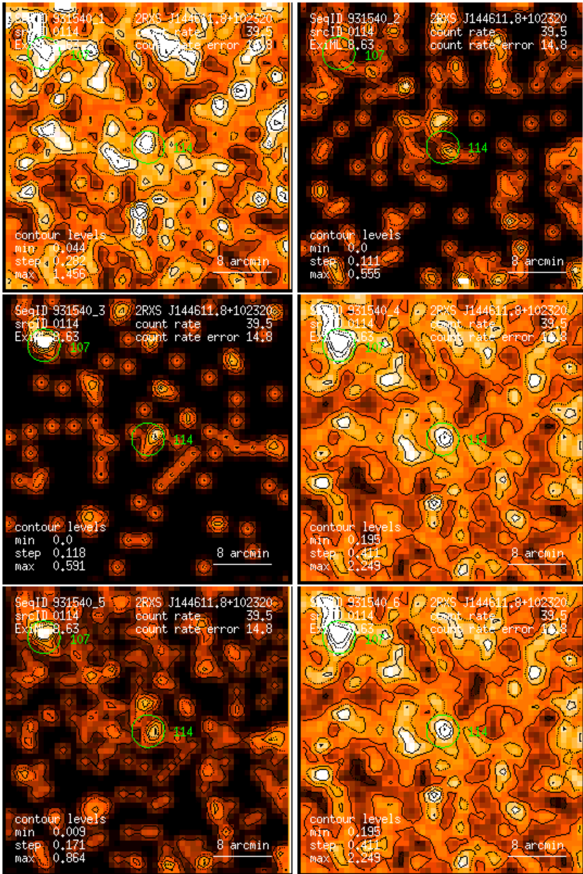
Figure 114: RASS 931540: detection 0114: band rate images, Gaussian filter: (1) PSPC channels 11 – 41, (2) 52 – 90, (3) 91 – 201, (4) 11 – 235, (5) 52 – 201, (6) 11 – 201. Broad band rates in counts/ks. Band rate contour levels in counts/ks/arcmin 2 .
